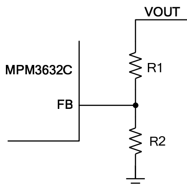
Figure 6: Feedback Network
