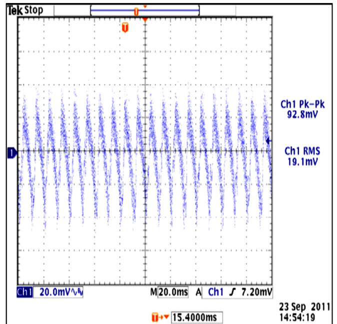
12V OUT, FULL LOAD, 230VAC, 60HZ
