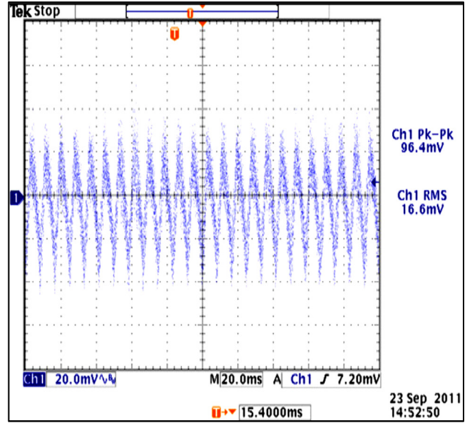
12V OUT, FULL LOAD, 115VAC, 60HZ
