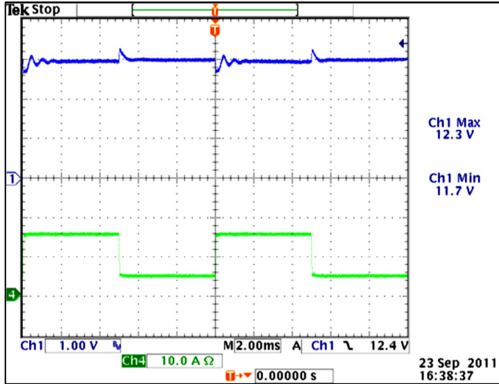
12V OUT, 115VAC, 25% TO 75% LOAD STEP
