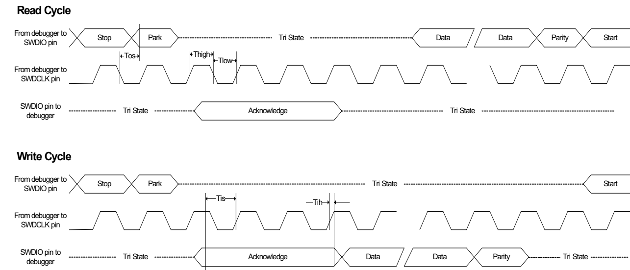
Figure 35-17.SWD Interface Signals
