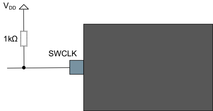
Figure 37-10.SWCLK Circuit Connections
