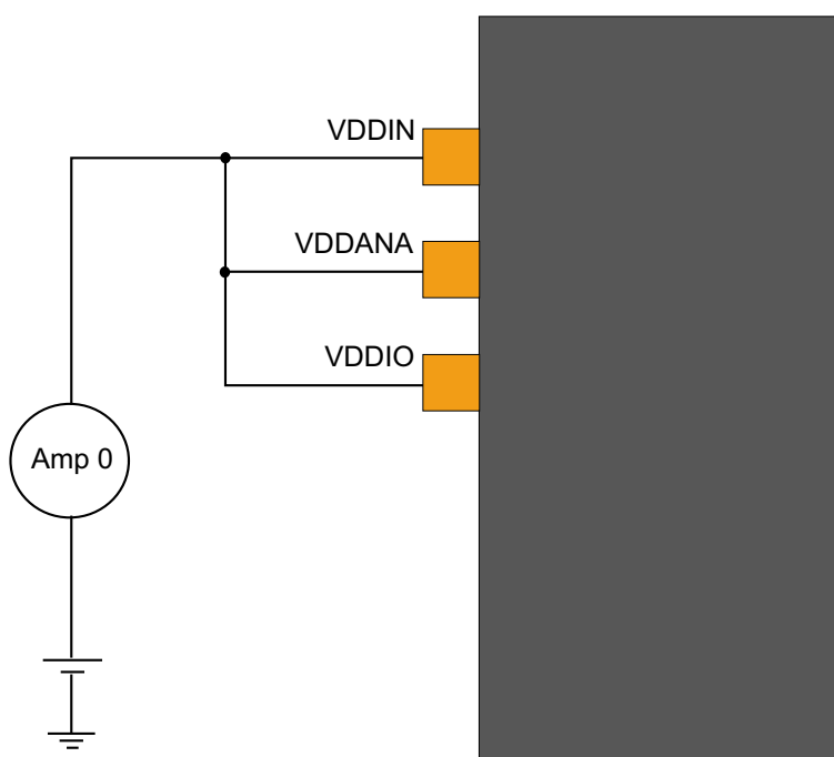
Figure 40-1. Measurement Schematic
