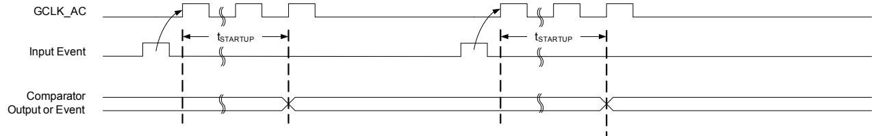
Figure 32-10. Single-Shot SleepWalking
