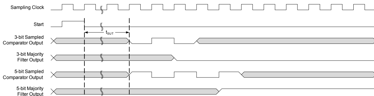
Figure 32-7. Single-Shot Filtering
