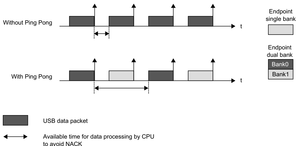
Figure 30-6. Ping-Pong Overview
