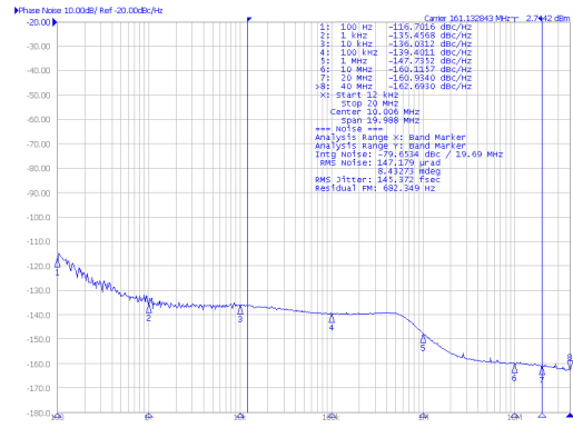
Figure 4. Closed-Loop Phase Noise of LVPECL Differential Output at 161.1328125 MHz
