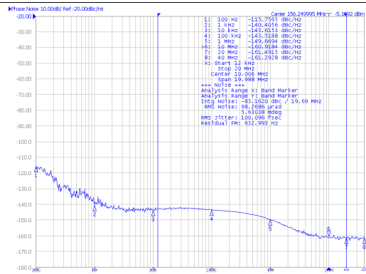
Figure 2. Closed-Loop Phase Noise of LVDS Differential Output at 156.25 MHz
