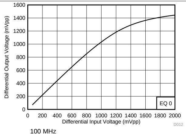
图 16. Upstream-to-Downstream Linearity Performance at 100 MHz
