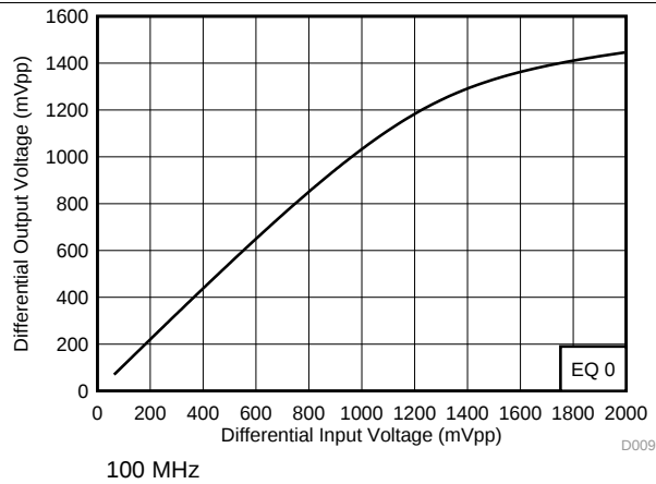
图 13. Downstream-to-Upstream Linearity Performance at 100 MHz
