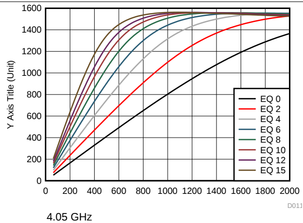
图 15. Upstream-to-Downstream Linearity Performance at 4.05 GHz
