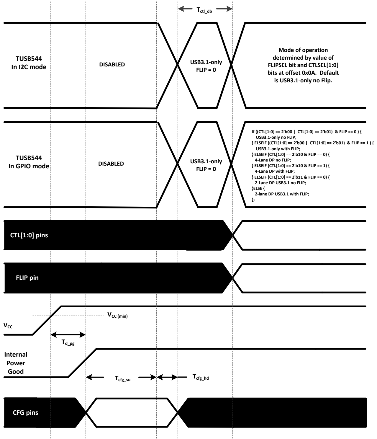
图 21. Power-Up Timing
