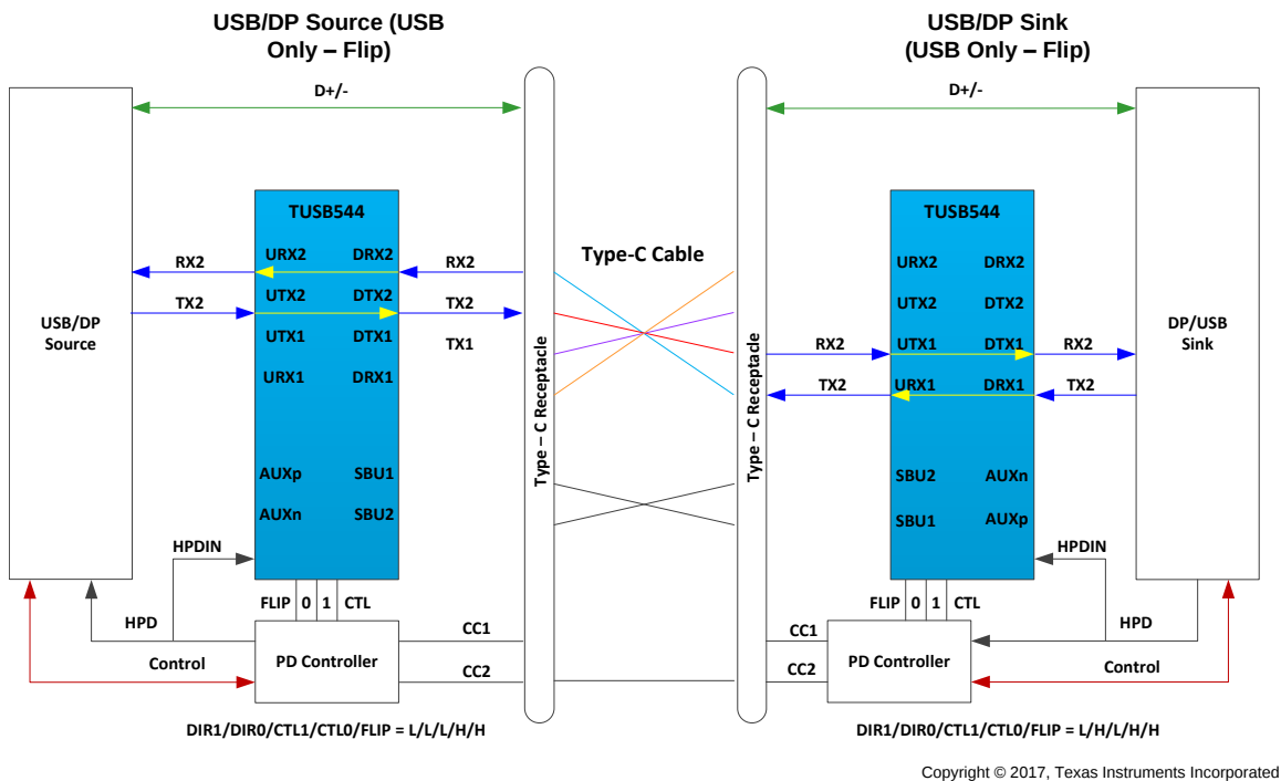
图 38. USB3.1 Only – With Flip
