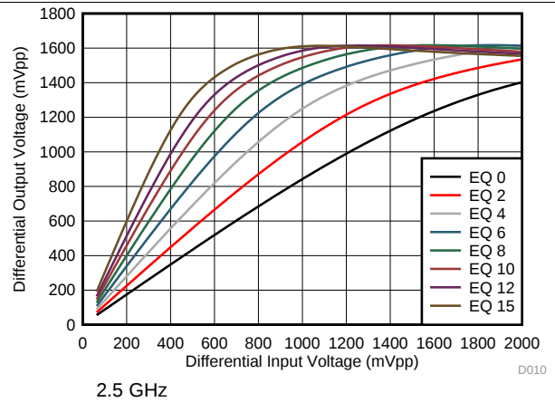
图 14. Upstream-to-Downstream Linearity Performance at 2.5 GHz
