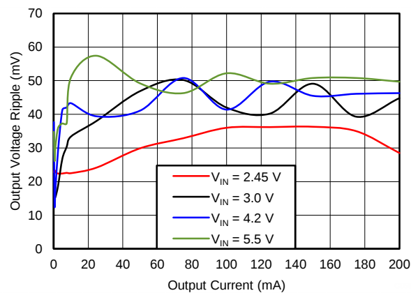
Figure 63. Output Voltage Ripple vs Output Current
