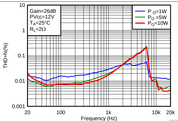
图 18. Total Harmonic Distortion + Noise (PBTL) vs Frequency
