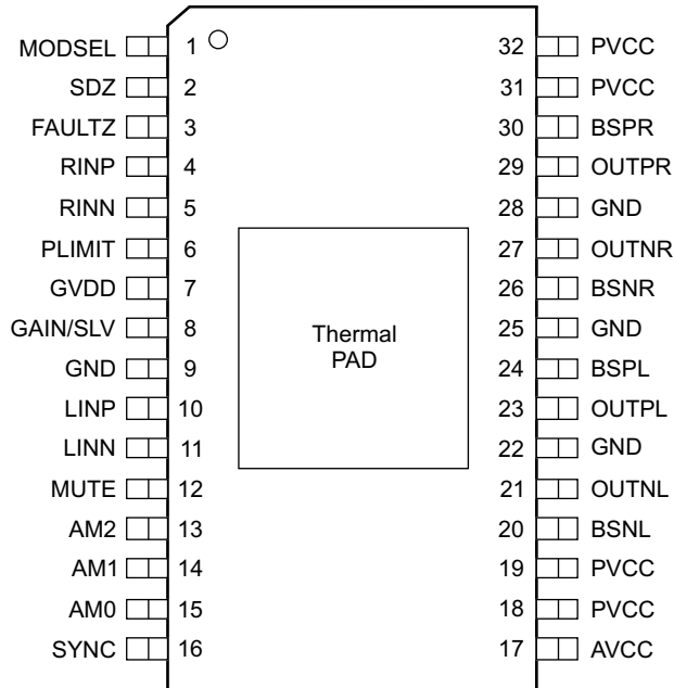
DAP Package 32-Pin HTSSOP With PowerPAD Down TPA3128D2, Top View
