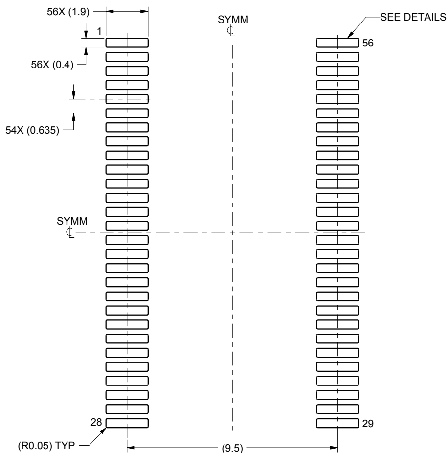
LAND PATTERN EXAMPLE SCALE:6X
