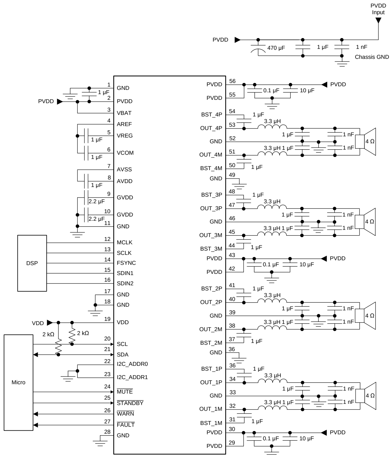
Figure 79. Typical 4-Channel BTL Application Schematic
