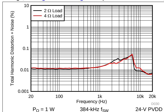
Figure 25. PBTL THD+N vs Frequency
