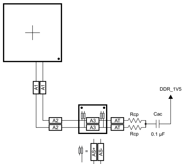
Figure 8-51. CK Routing for Two Mirrored DDR3 Devices
