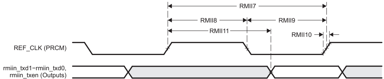
Figure 7-52. GMAC Transmit Interface Timing RMII n Operation
