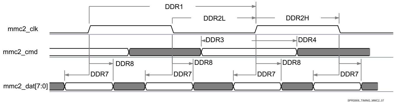
Figure 7-74. MMC/SD/SDIO in - High Speed DDR JC64 - Receiver Mode
