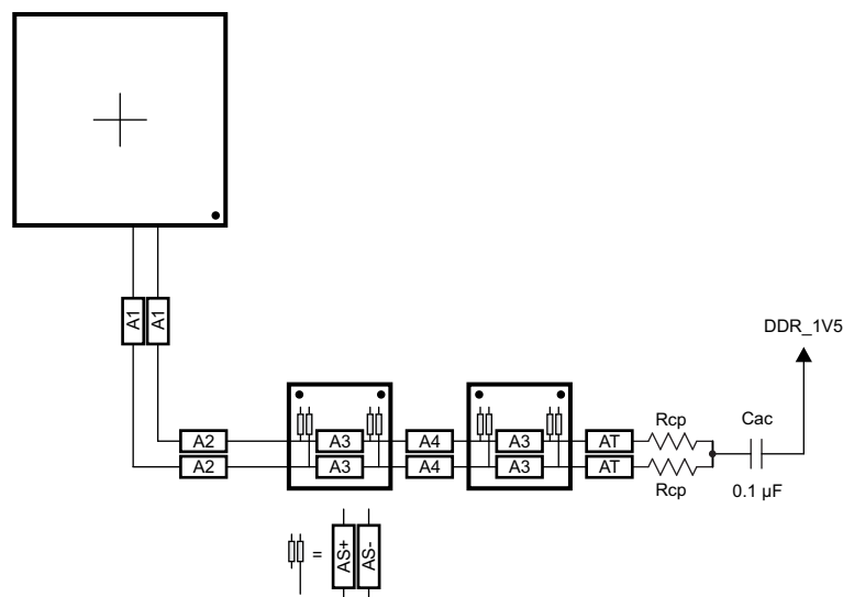
Figure 8-45. CK Routing for Four Mirrored DDR3 Devices
