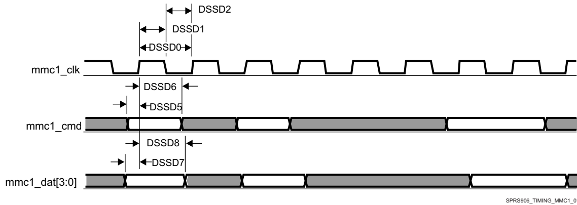
Figure 7-55. MMC/SD/SDIO in - Default Speed - Receiver Mode
