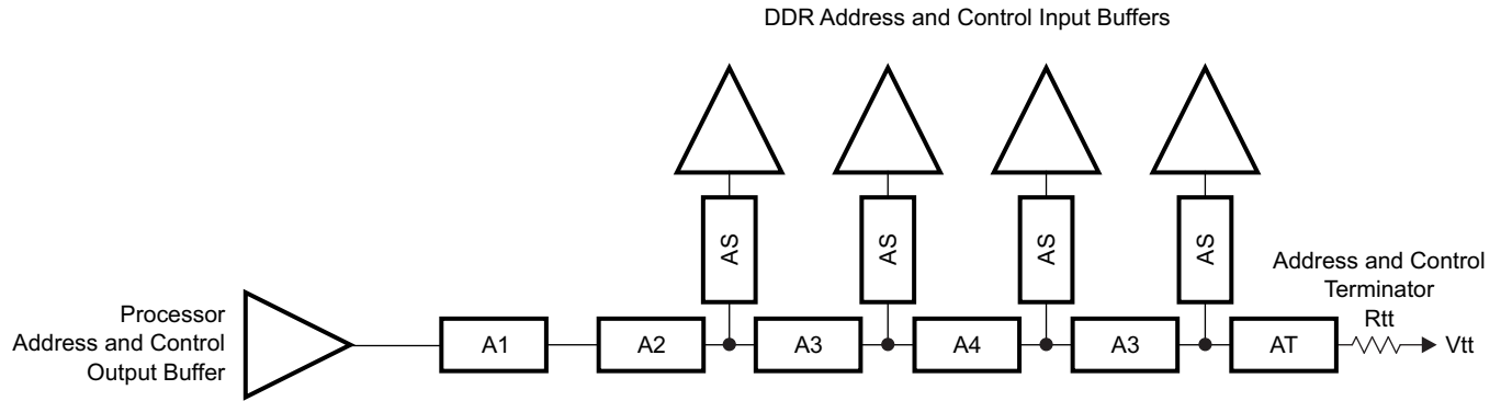
Figure 8-42. ADDR_CTRL Topology for Four x8 DDR3 Devices
