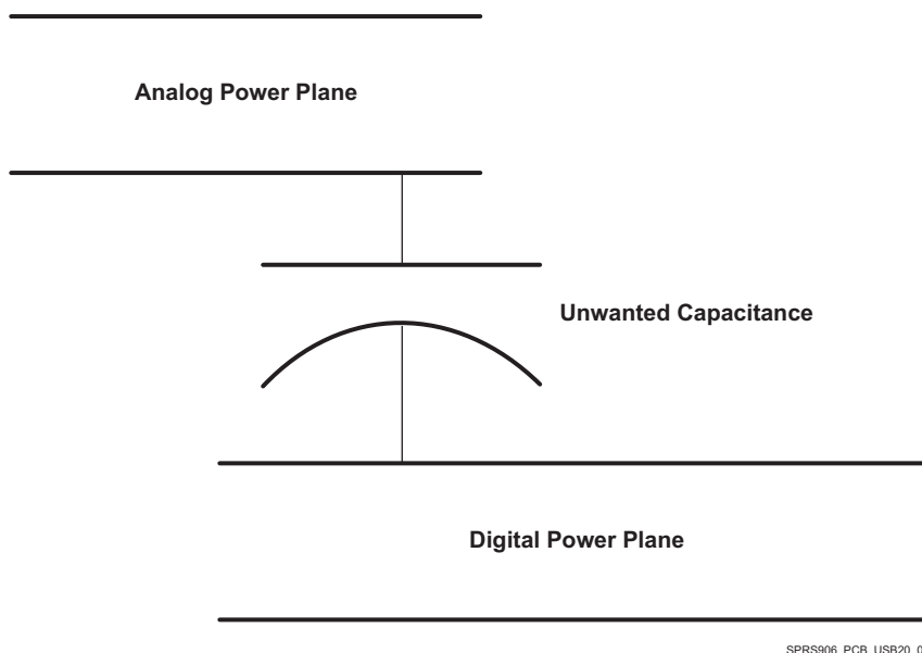
Figure 8-28. Do Not Overlap Planes
