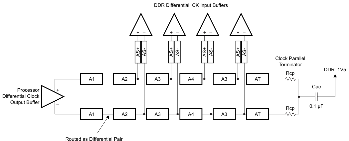
Figure 8-41. CK Topology for Four x8 DDR3 Devices
