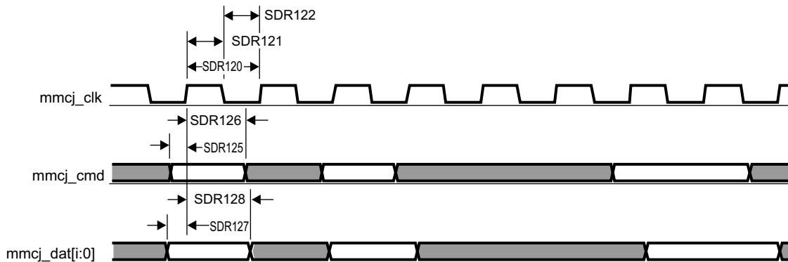
Figure 7-80. MMC/SD/SDIOj in - SDR12 - Receiver Mode
