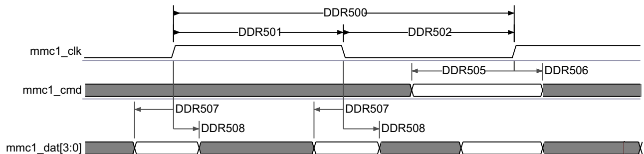
Figure 7-67. SDMMC - High Speed SD - DDR - Data/Command Receive
