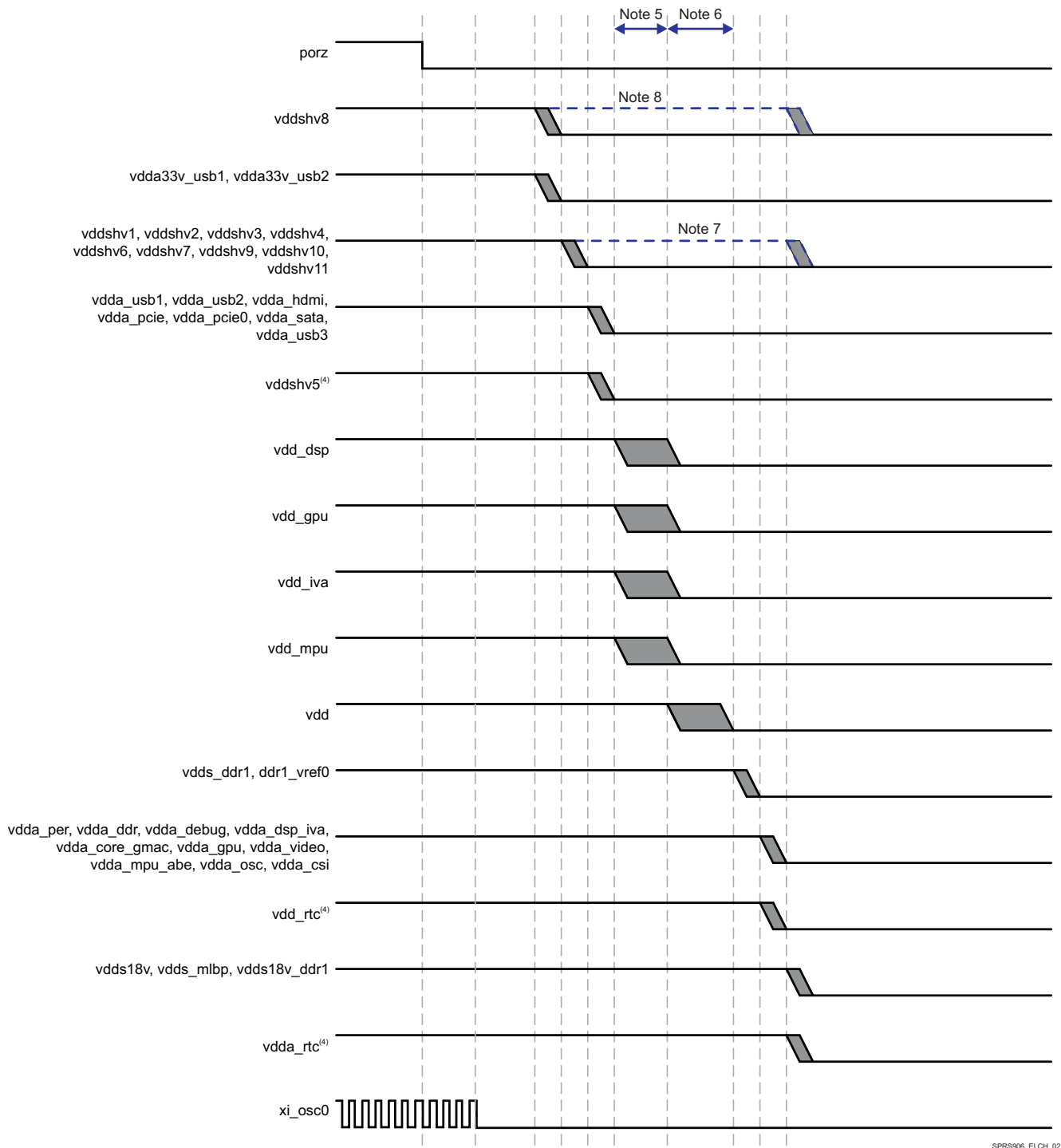
Figure 5-2. Power-Down Sequencing
