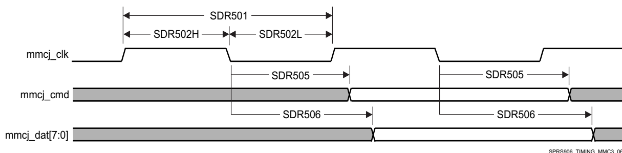
Figure 7-85. MMC/SD/SDIOj in - High Speed SDR50 - Transmitter Mode
