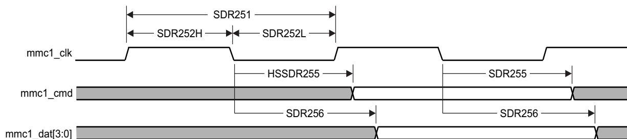
Figure 7-62. MMC/SD/SDIO in - High Speed SDR25 - Transmitter Mode
