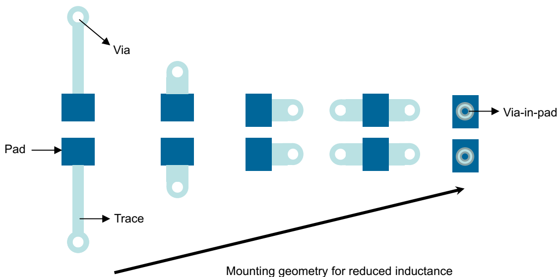
Figure 8-9. Capacitor Placement Geometry for Improved Mounting Inductance
