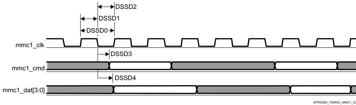
Figure 7-56. MMC/SD/SDIO in - Default Speed - Transmitter Mode
