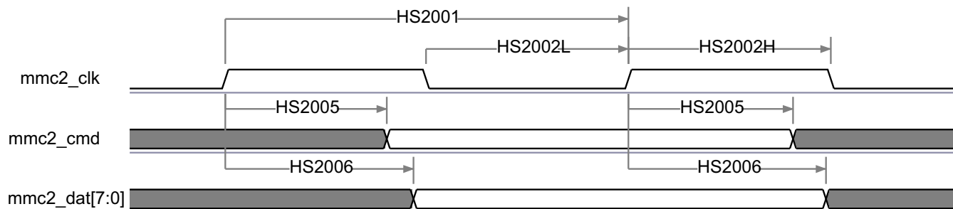
Figure 7-73. eMMC in - HS200 SDR - Transmitter Mode
