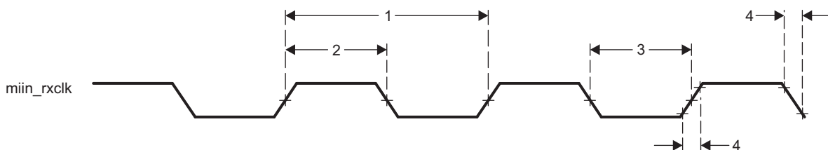
Figure 7-46. Clock Timing (GMAC Receive) - MII in operation
