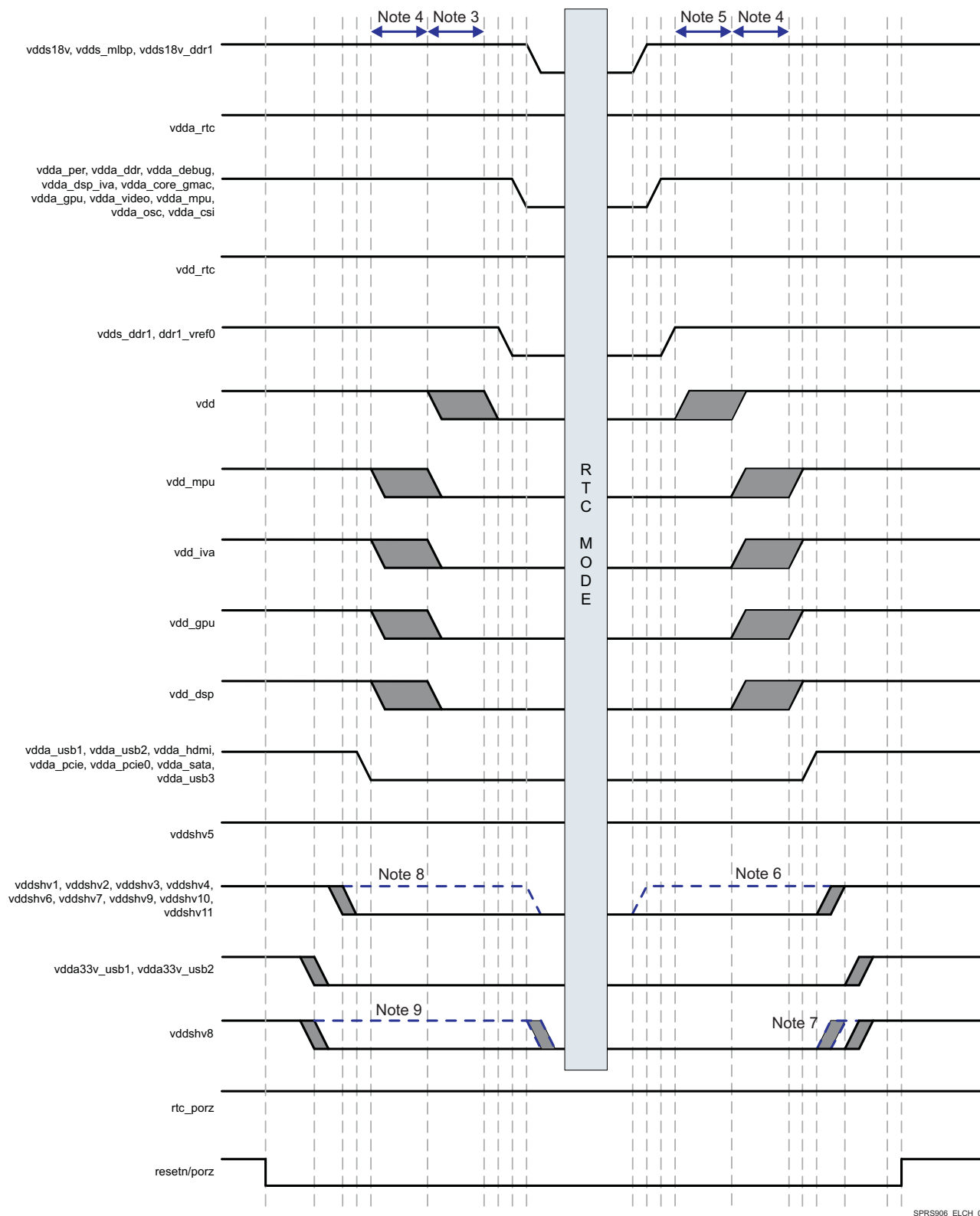
Figure 5-3. RTC Mode Sequencing
