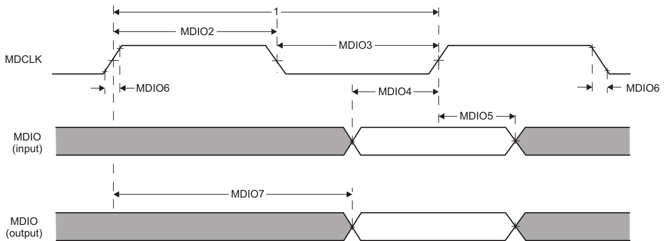
Figure 7-50. GMAC MDIO diagrams
