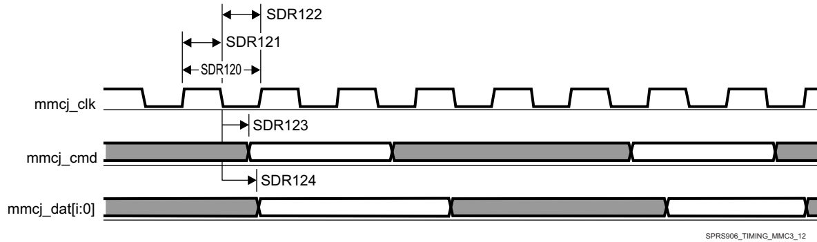
Figure 7-81. MMC/SD/SDIOj in - SDR12 - Transmitter Mode
