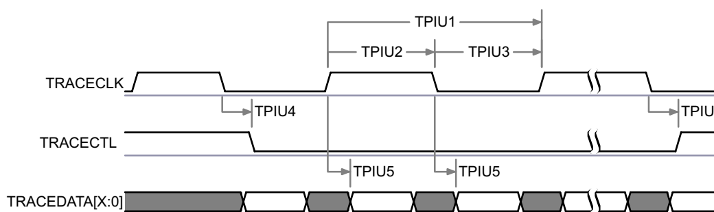
Figure 7-88. TPIU-PLL DDR Transmit Mode (1)
