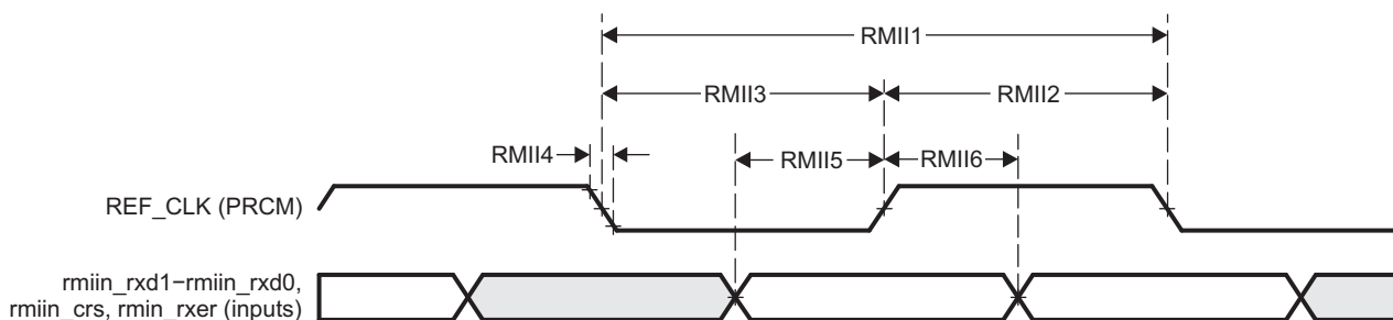
Figure 7-51. GMAC Receive Interface Timing RMIIn operation
