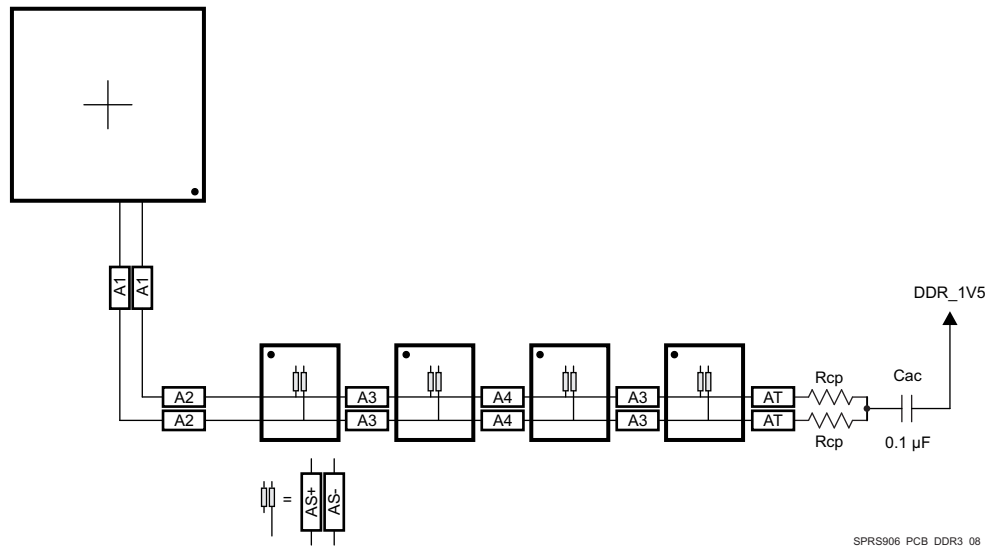
Figure 8-43. CK Routing for Four Single-Side DDR3 Devices
