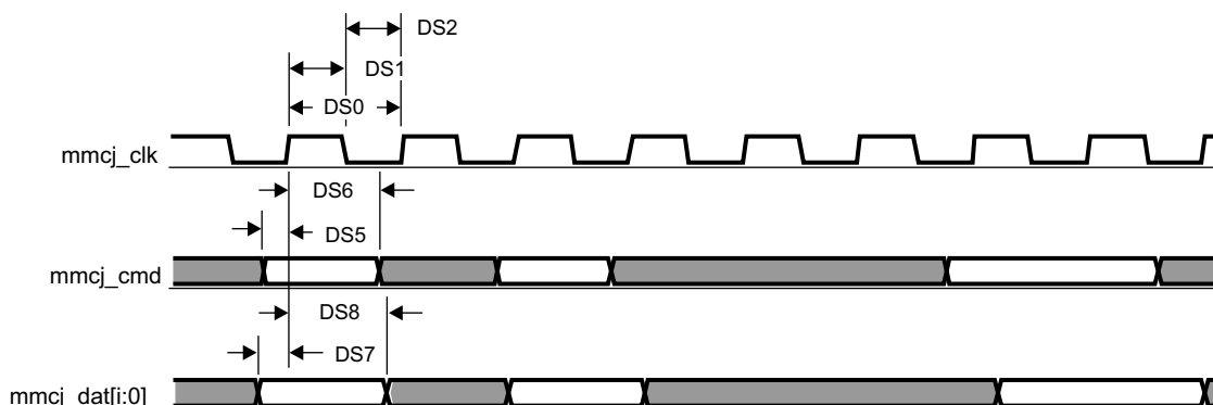
Figure 7-76. MMC/SD/SDIOj in - Default Speed - Receiver Mode
