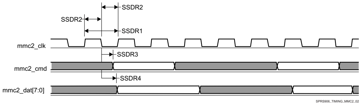
Figure 7-70. MMC/SD/SDIO in - Standard JC64 - Transmitter Mode
