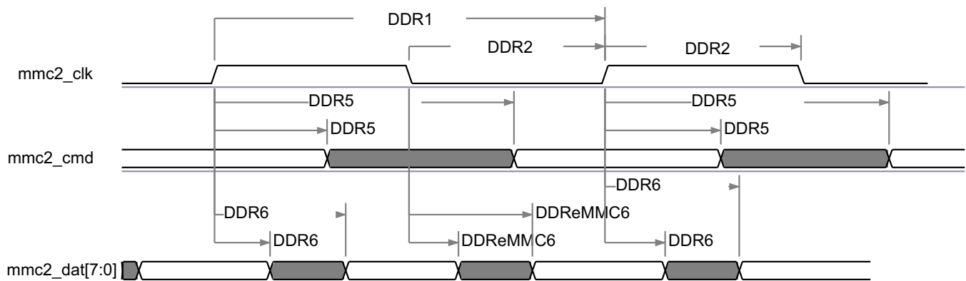
Figure 7-75. MMC/SD/SDIO in - High Speed DDR JC64 - Transmitter Mode
