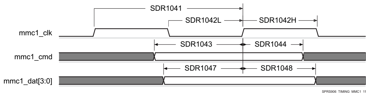
Figure 7-65. MMC/SD/SDIO in - High Speed SDR104 - Receiver Mode
