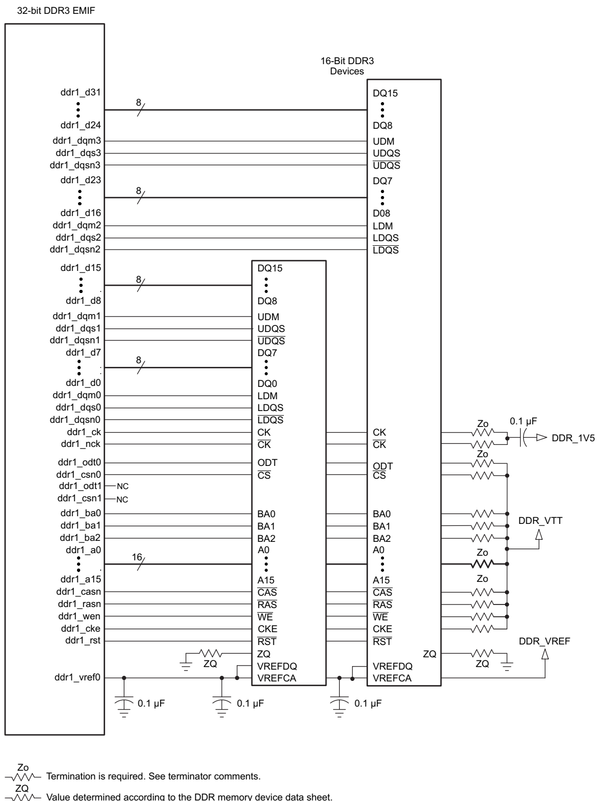
Figure 8-37. 32-Bit, One-Bank DDR3 Interface Schematic Using Two 16-Bit DDR3 Devices
