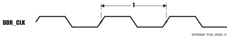
Figure 8-36. DDR3 Memory Controller Clock Timing
