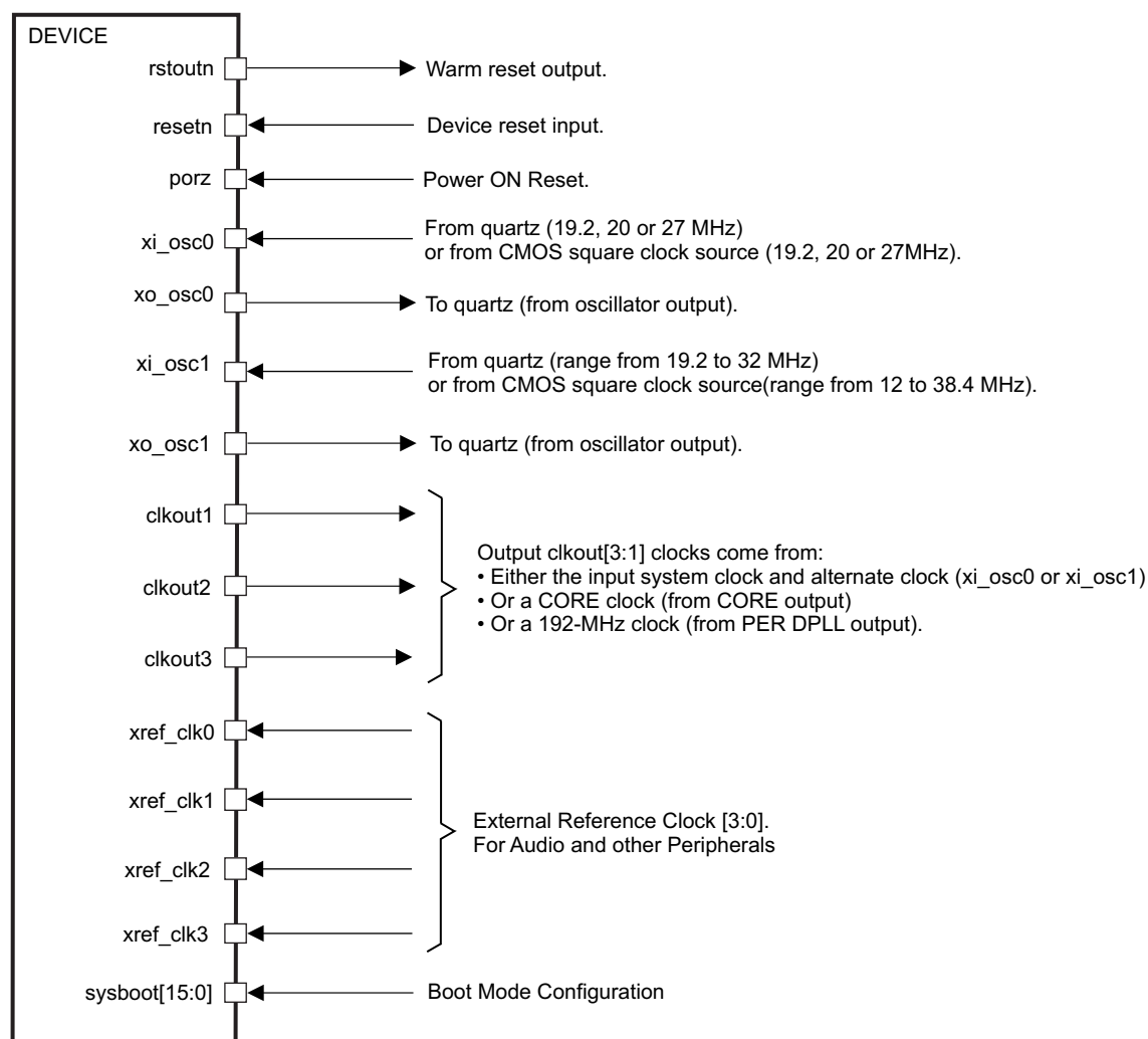
Figure 6-1. Clock Interface
