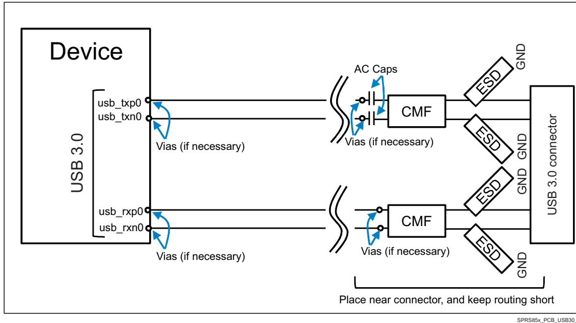
Figure 8-30. USB 3.0 Interface High Level Schematic
