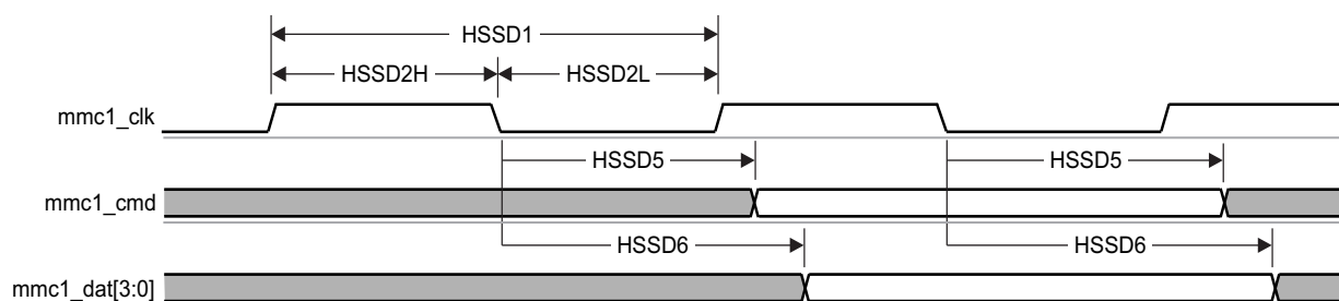
Figure 7-58. MMC/SD/SDIO in - High Speed - Transmitter Mode
