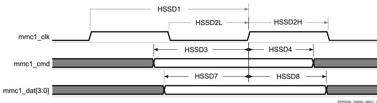
Figure 7-57. MMC/SD/SDIO in - High Speed - Receiver Mode
