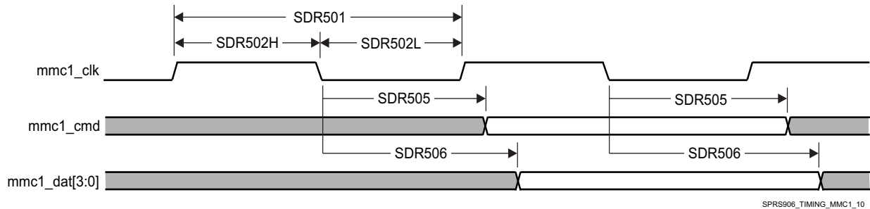
Figure 7-64. MMC/SD/SDIO in - High Speed SDR50 - Transmitter Mode
