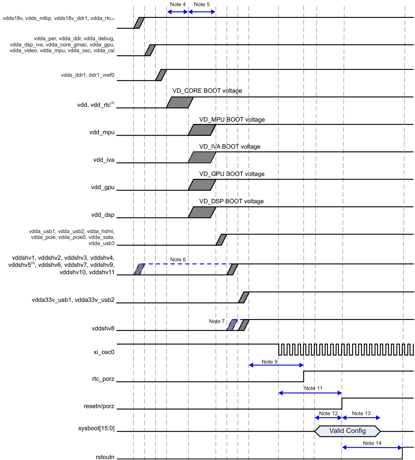
Figure 5-4. Power-Up Sequencing
