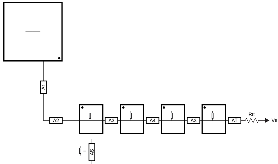
Figure 8-44. ADDR_CTRL Routing for Four Single-Side DDR3 Devices
