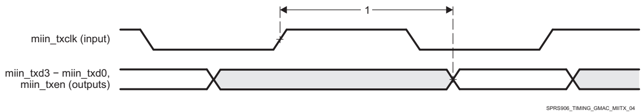
Figure 7-49. GMAC Transmit Interface Timing MII operation
