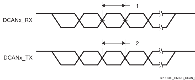
Figure 7-45. DCANx Timings
