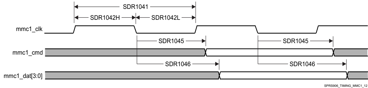
Figure 7-66. MMC/SD/SDIO in - High Speed SDR104 - Transmitter Mode
