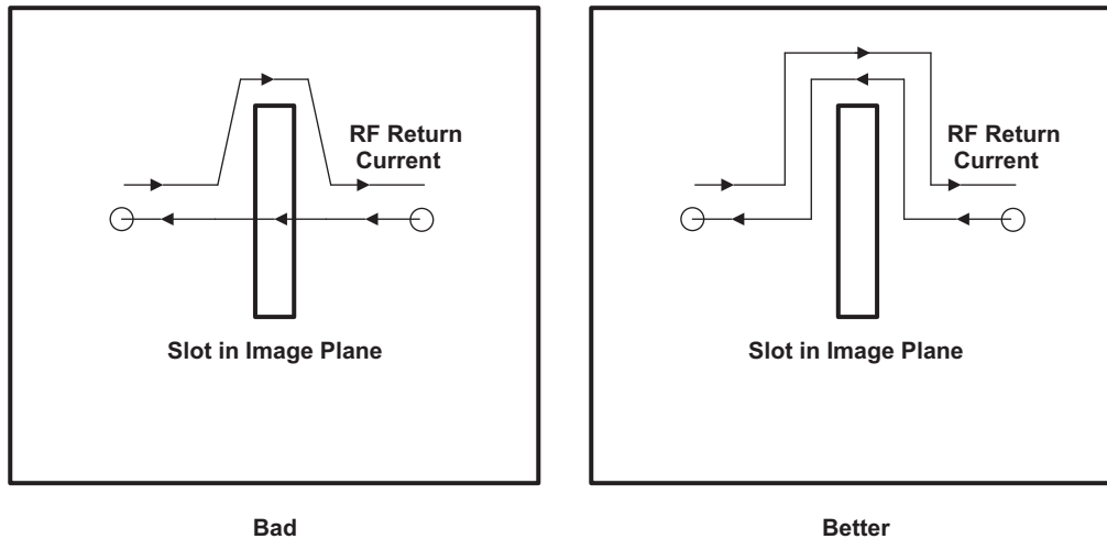
Figure 8-29. Do Not Violate Image Planes
