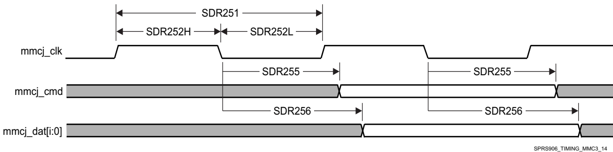
Figure 7-83. MMC/SD/SDIOj in - SDR25 - Transmitter Mode
