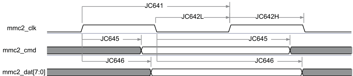
Figure 7-72. MMC/SD/SDIO in - High Speed JC64 - Transmitter Mode
