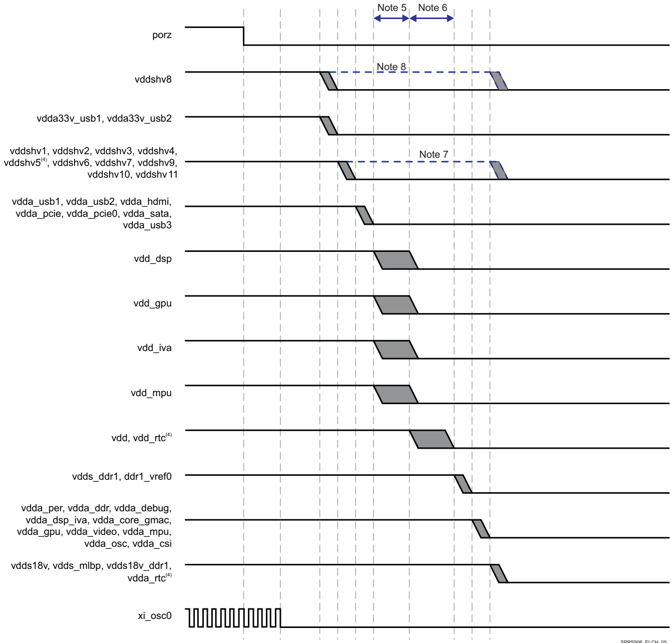
Figure 5-5. Power-Down Sequencing
