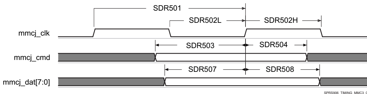
Figure 7-84. MMC/SD/SDIOj in - High Speed SDR50 - Receiver Mode
