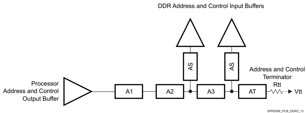
Figure 8-48. ADDR_CTRL Topology for Two DDR3 Devices
