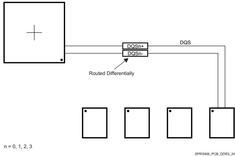
Figure 8-59. DQS Routing With Any Number of Allowed DDR3 Devices
