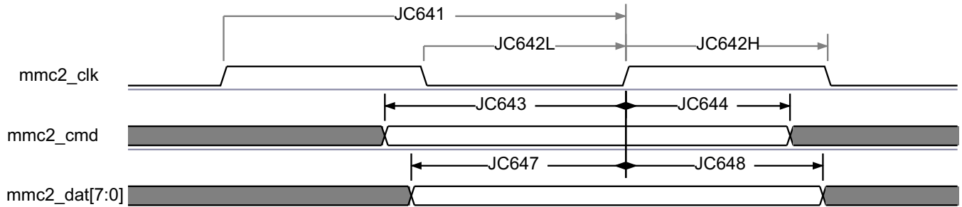
Figure 7-71. MMC/SD/SDIO in - High Speed JC64 - Receiver Mode
