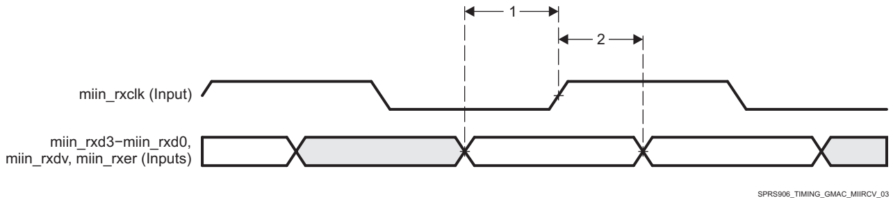
Figure 7-48. GMAC Receive Interface Timing MII operation
