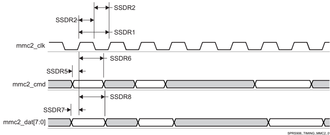
Figure 7-69. MMC/SD/SDIO in - Standard JC64 - Receiver Mode
