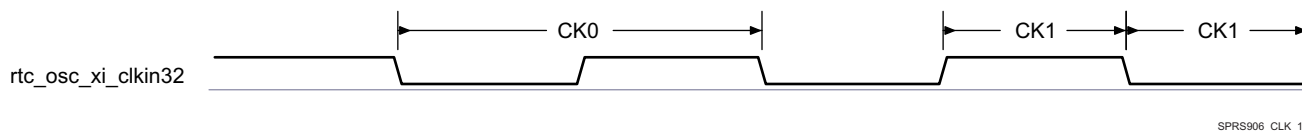
Figure 6-13. rtc_osc_xi_clkin32 Input Clock
