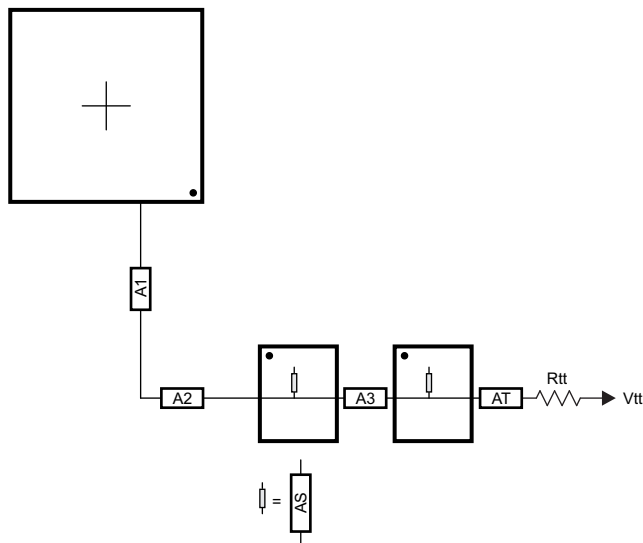
Figure 8-50. ADDR_CTRL Routing for Two Single-Side DDR3 Devices
