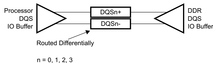
Figure 8-57. DQS Topology
