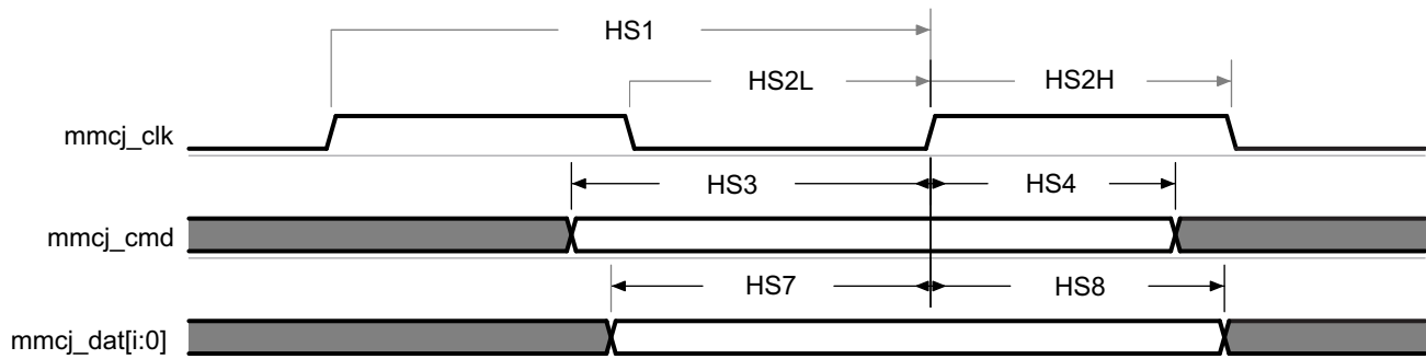
Figure 7-78. MMC/SD/SDIOj in - High Speed - Receiver Mode
