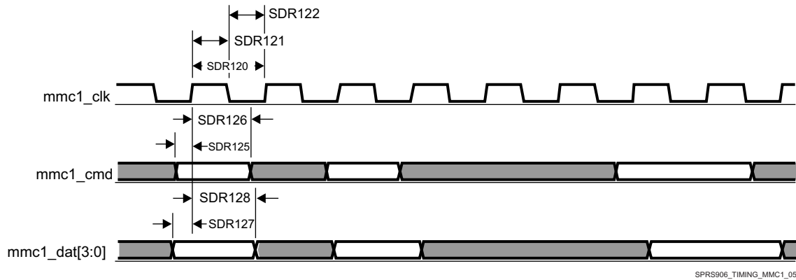
Figure 7-59. MMC/SD/SDIO in - High Speed SDR12 - Receiver Mode
