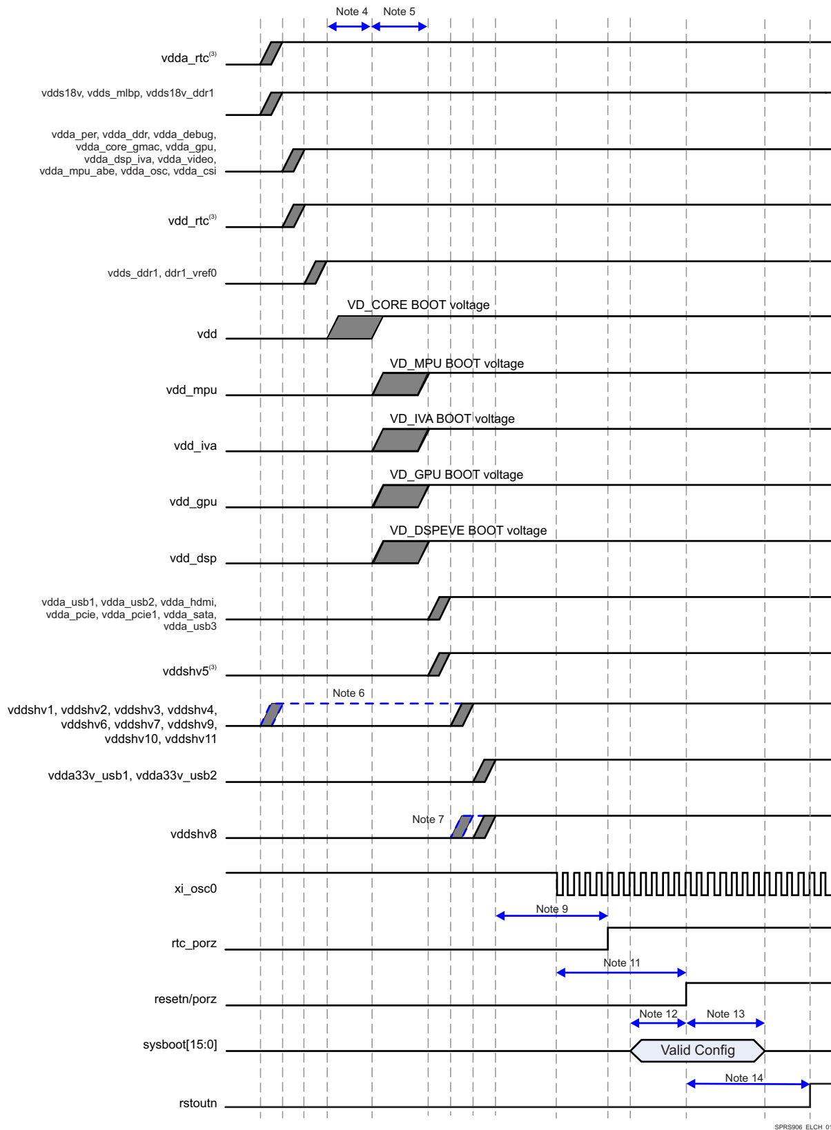
Figure 5-1. Power-Up Sequencing
