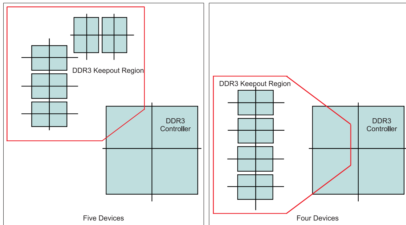
Figure 8-40. DDR3 Keepout Region
