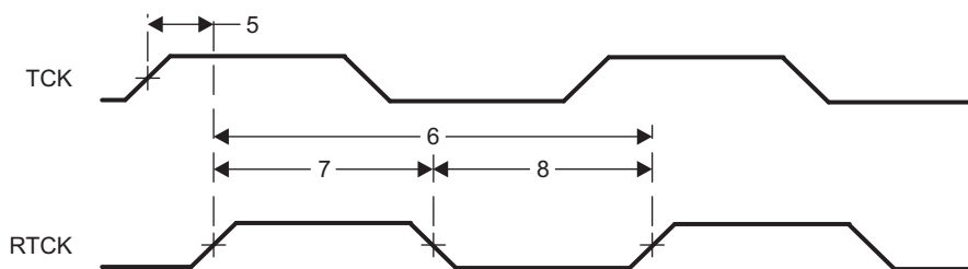
Figure 7-87. JTAG With RTCK Timing
