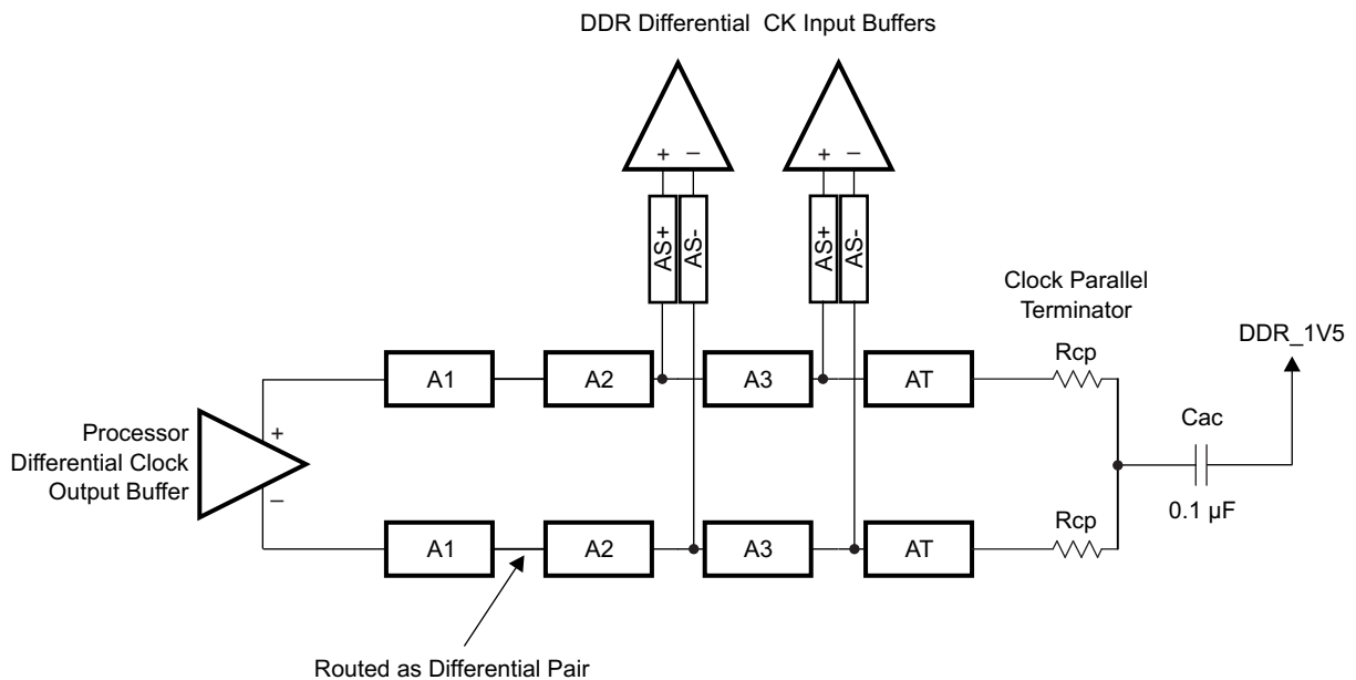
Figure 8-47. CK Topology for Two DDR3 Devices
