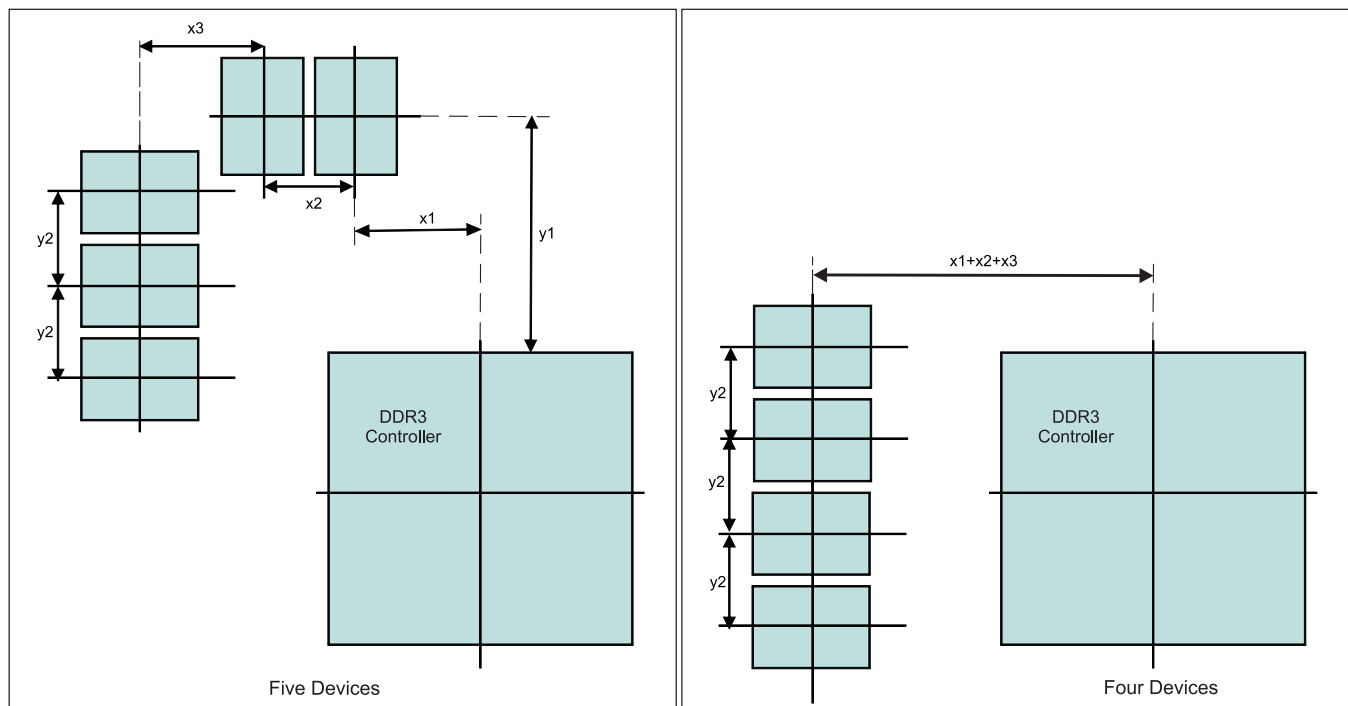
Figure 8-39. Placement Specifications
