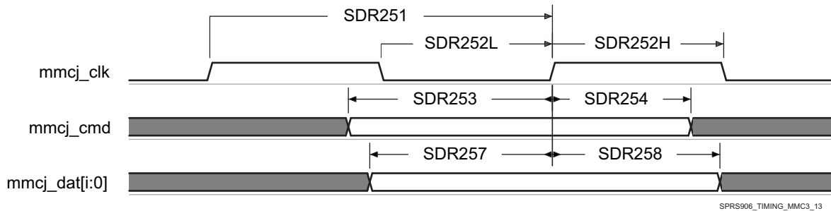
Figure 7-82. MMC/SD/SDIOj in - SDR25 - Receiver Mode
