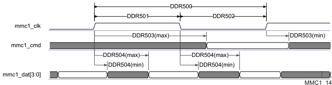
Figure 7-68. SDMMC - High Speed SD - DDR - Data/Command Transmit
