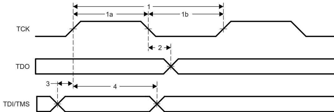
Figure 7-86. JTAG Timing
