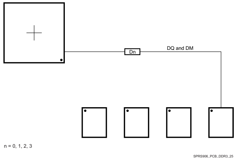
Figure 8-60. DQ/DM Routing With Any Number of Allowed DDR3 Devices
