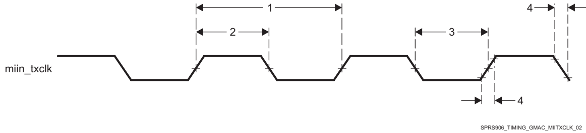
Figure 7-47. Clock Timing (GMAC Transmit) - MII operation
