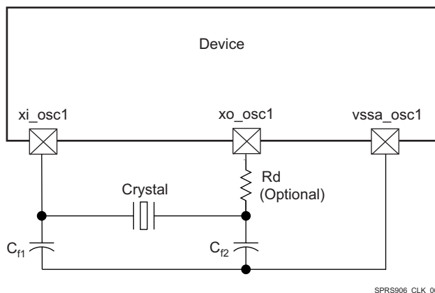
Figure 6-6. Crystal Implementation
