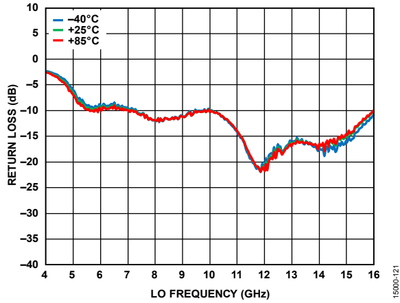
Figure 31. LO Return Loss vs. LO Frequency at Various Temperatures
