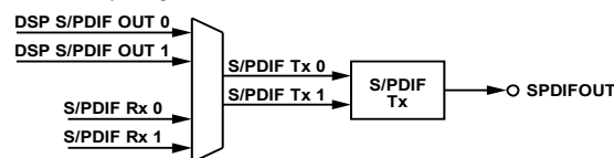
Figure 49. S/PDIF Transmitter Source Selection
