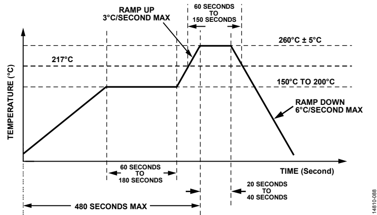
Figure 92. Soldering Profile
