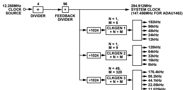
Figure 18. PLL and Audio Clock Generators with Default Settings and Resulting Clock Frequencies Labeled, XTALIN/MCLK = 12.288 MHz
