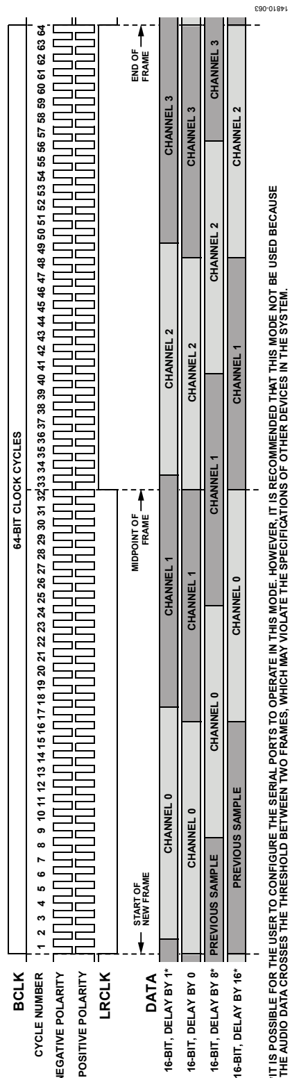
Figure 65. Serial Audio Data Formats; Four Channels, 16 Bits per Channel
