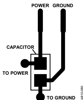
Figure 84. Recommended Power Supply Bypass Capacitor Layout
