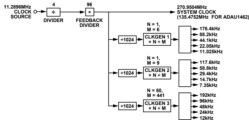
Figure 19. PLL and Audio Clock Generators with Default Settings and Resulting Clock Frequencies Labeled, XTALIN/MCLK = 11.2896 MHz
