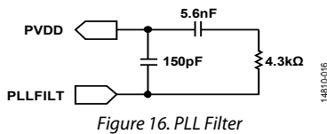
Figure 16. PLL Filter
