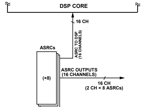
Figure 60. ASRC Outputs
