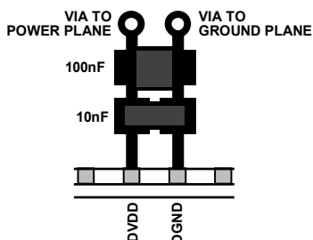
Figure 85. Layout for Multiple Power Supply Bypass Capacitors
