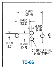
TO-66
