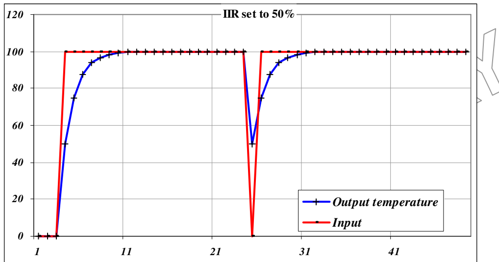
Fig. 9 IIR set to 50% response to step and spike
