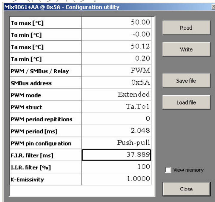
Fig. 7 MLX90614 configured for higher speed, filters set to minimum, Extended PWM output Tamb, Tobj, period 2ms (500 Hz pulse train), push-pull output. Temperature range set to 0..+50 °C.
