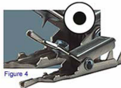
The single-needle style clip is for single penetration of heavier wire.
