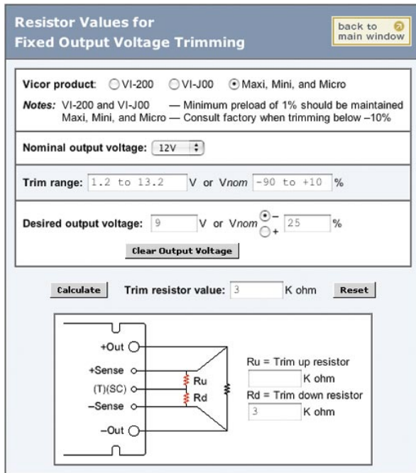
Figure 2-16 — Online trim calculator
