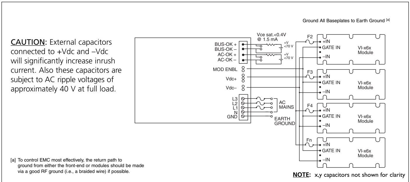
Figure 16-4 — 5.0 kW Front-end
