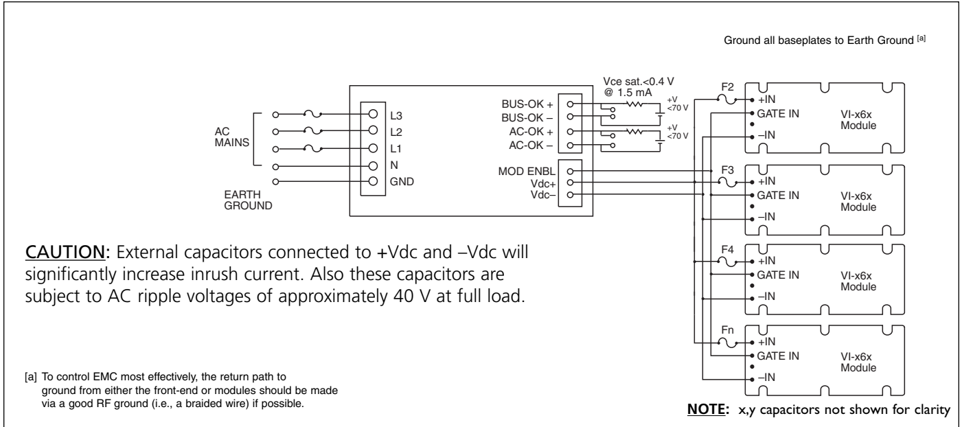
Figure 16-3 — 1.5, 3.0 kW Front-end
