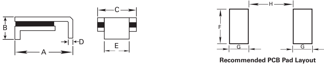
Recommended PCB Pad Layout
