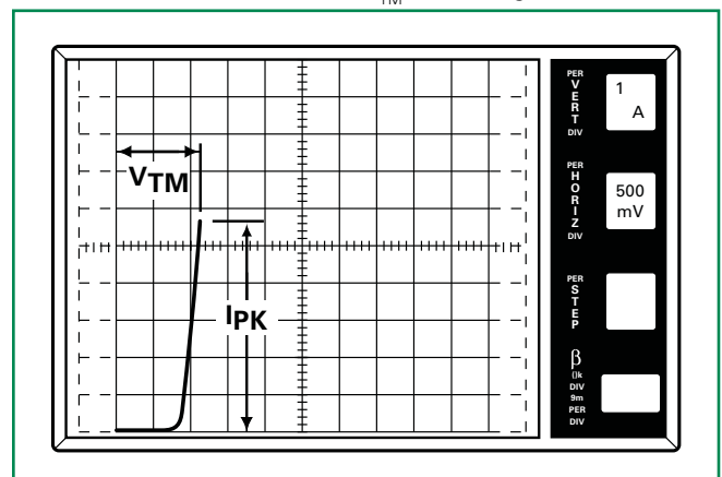
Figure AN1006.20 V_{TM} (Forward) = 1.1 V at I_{PK} = 5.6 \text{ A}
