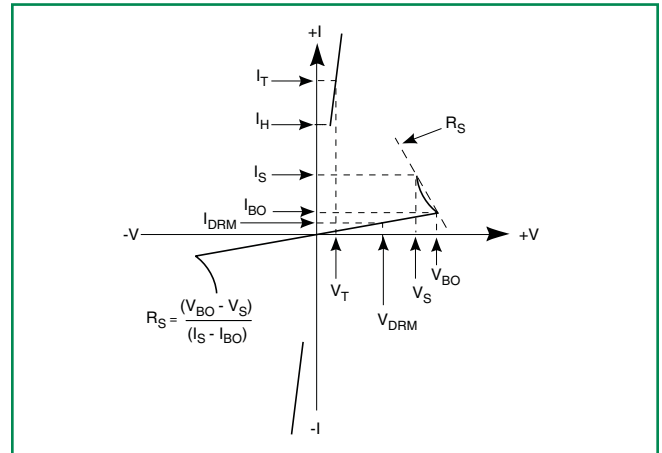
V-I Characteristics of SIDAC Device with Negative Resistance
