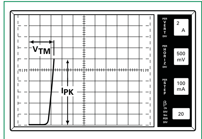
Figure AN1006.7 V_{TM} = 1.15 \text{ V} at I_{T(peak)} = 12 \text{ A}
