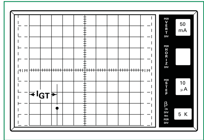
Figure AN1006.9 I_{GT} = 25 \mu\text{A}
