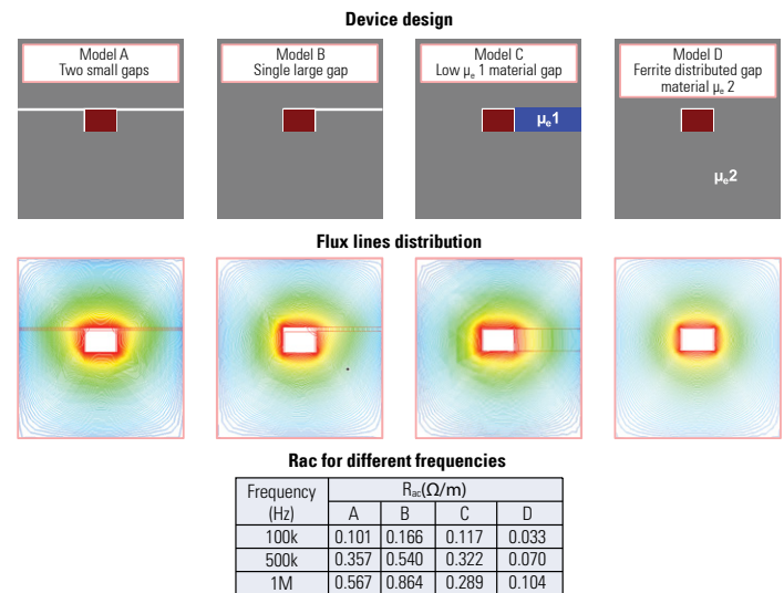
Figure 2. Modeling is one of Eaton's Electronics Division tools for providing higher efficiency inductors.
