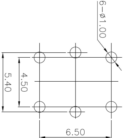
PCBLayout(Pattern Side)
