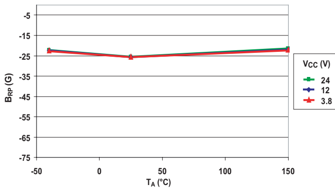
Release Point versus Ambient Temperature (A1202, A1203)
