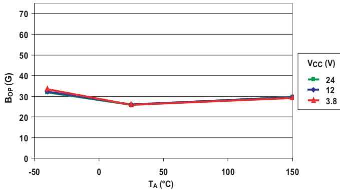
Operate Point versus Ambient Temperature (A1202, A1203)
