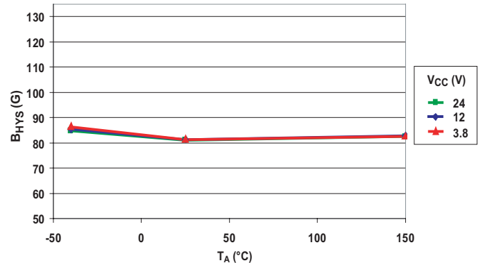
Hysteresis versus Ambient Temperature (A1204)
