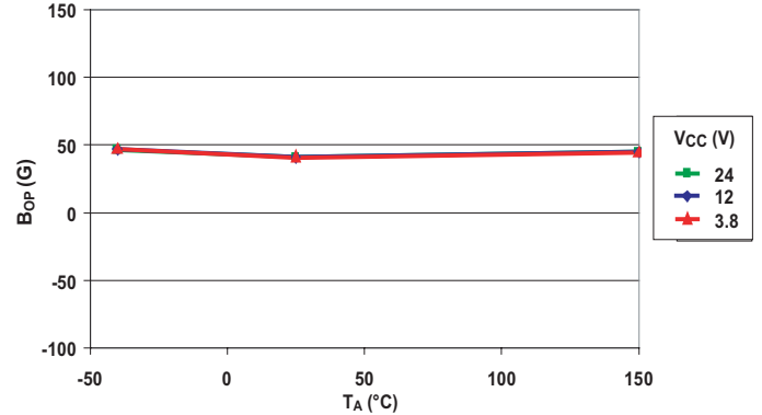
Operate Point versus Ambient Temperature (A1204)
