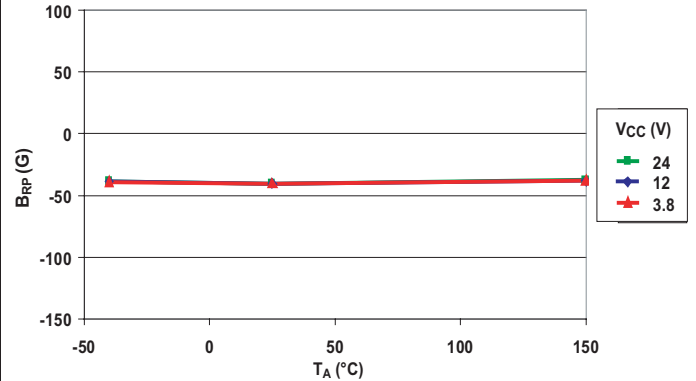
Release Point versus Ambient Temperature (A1204)
