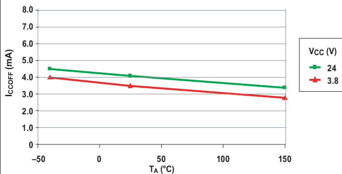
Supply Current (Off) versus Ambient Temperature (A1201/02/03/04)
