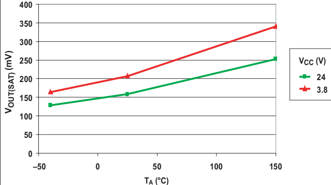
Output Voltage (On) versus Ambient Temperature (A1201/02/03/04)
