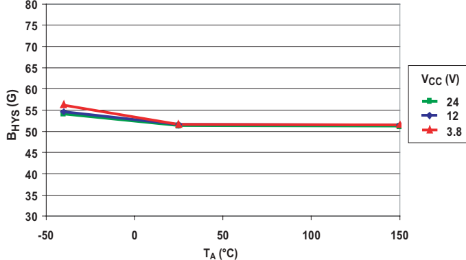
Hysteresis versus Ambient Temperature (A1202, A1203)
