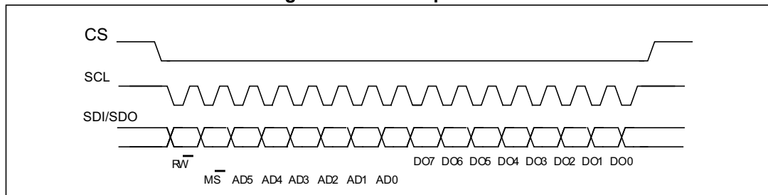
Figure 5. SPI read protocol
