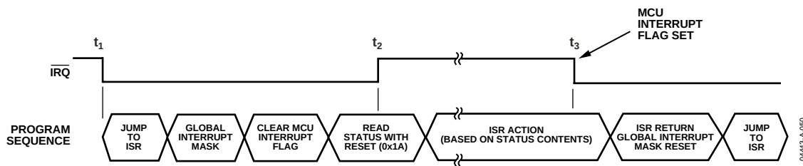
Figure 87. ADE7758 Interrupt Management
