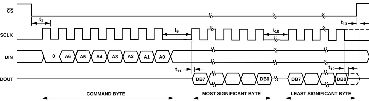
Figure 4. Serial Read Timing
