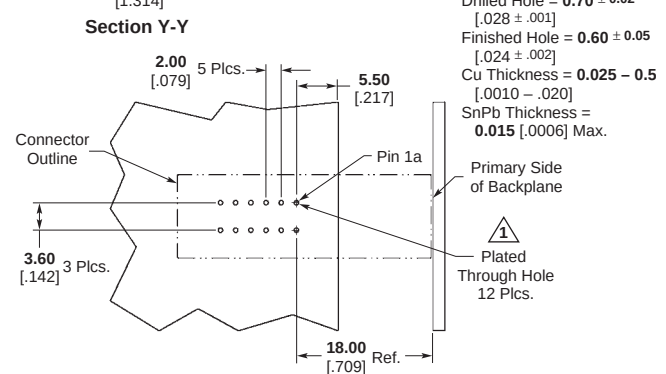
Recommended PCB Hole Layout
