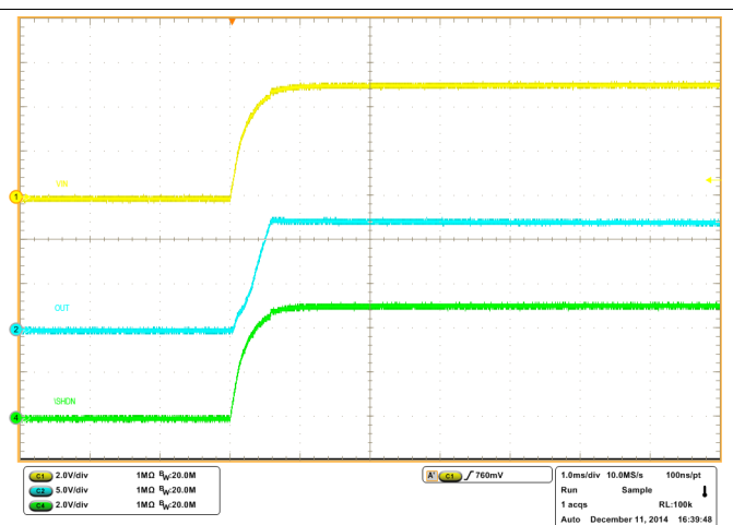
Figure 19. Typical Startup Waveform for V_{in} = 5.0 \text{ V} , V_{out} = 12 \text{ V}
