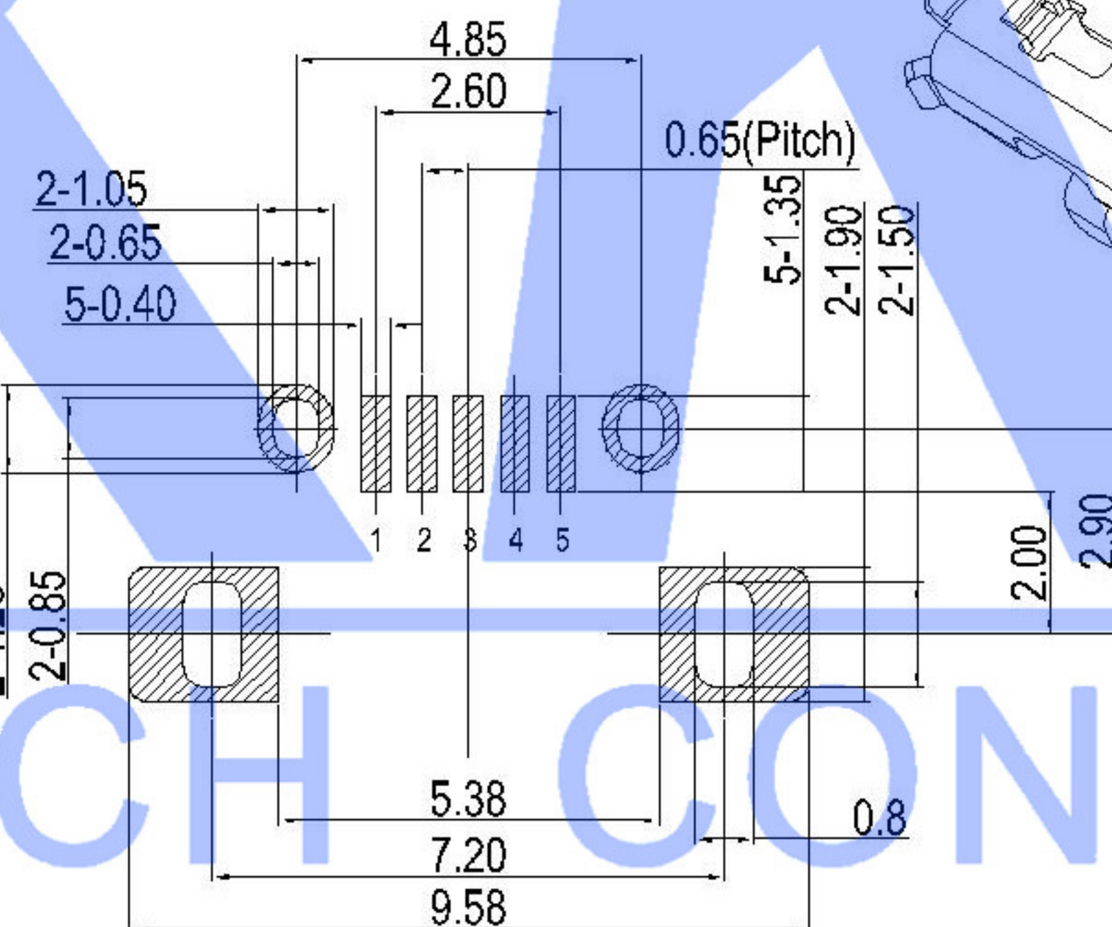
RECOMMENDED PCB LAYOUT(TOP VIEW)
