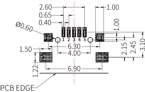
P.C.B LAYOUT(copper-side view)
