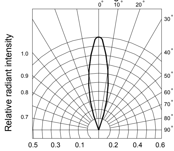
Radiation diagram
