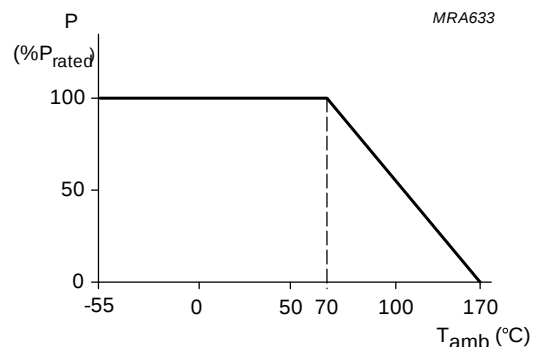
Fig. 6-2 Maximum dissipation (P max ) in percentage of rated power as a function of the operating ambient temperature (T amb )
