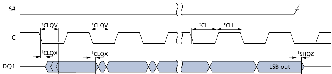
Figure 53: Output Timing
