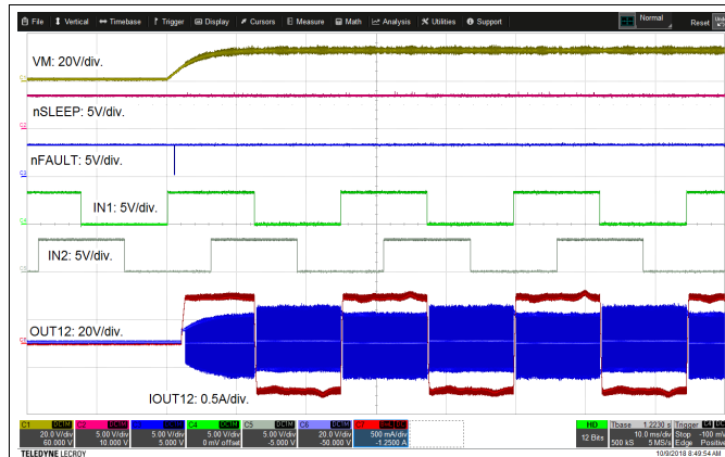
Figure 46. Device Power-up with Supply Voltage (VM)
