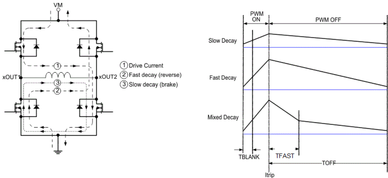
Figure 7-6. Decay Modes
