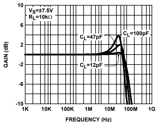
FIGURE 2. FREQUENCY RESPONSE FOR VARIOUS C_{LOAD}
