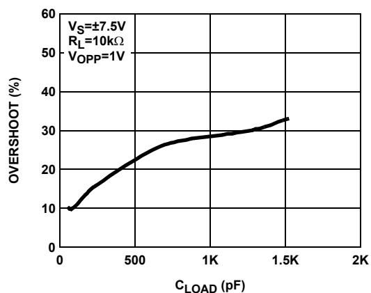
FIGURE 8. OVERSHOOT vs CAPACITANCE LOAD
