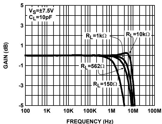
FIGURE 1. FREQUENCY RESPONSE FOR VARIOUS R_{LOAD}
