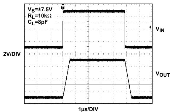
FIGURE 3. LARGE SIGNAL TRANSIENT RESPONSE
