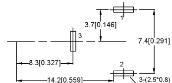
P.C.B LAYOUT (top view)
