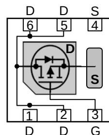
DFN2×2-6L
