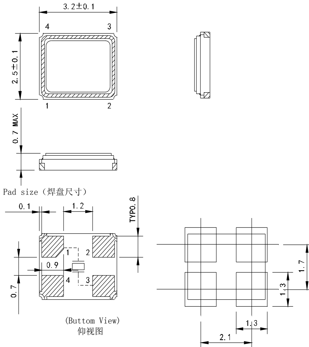
suggested solder pad layout
