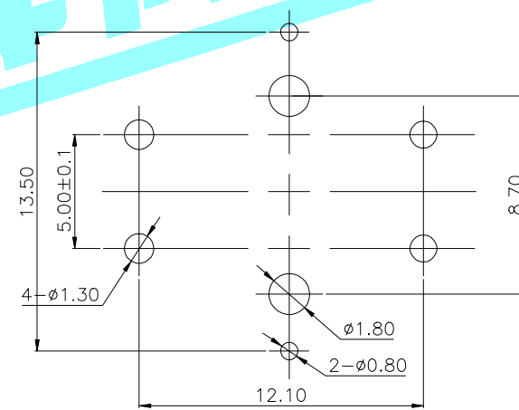
PCBLayout(pattern Side)
