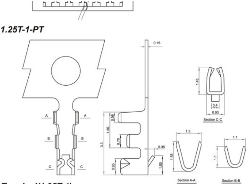
Terminal(1.25T-1)
