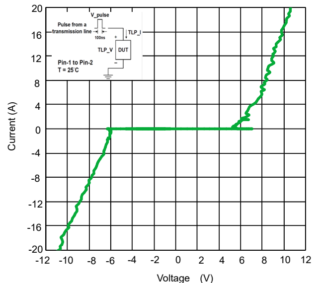
Fig 6. TLP Measurement
