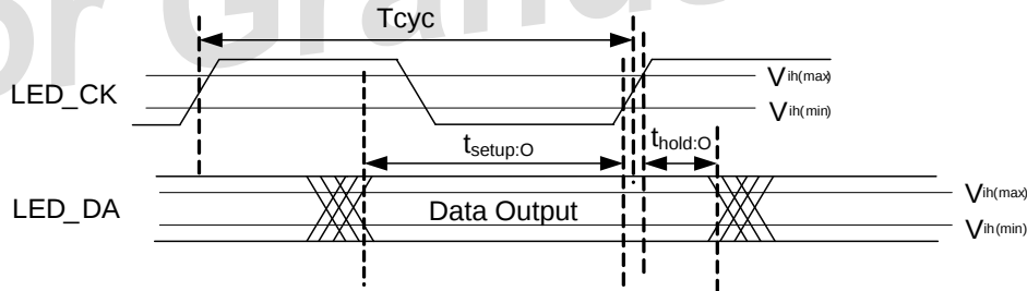
Figure 40. Serial Mode LED AC Timing Parameters
