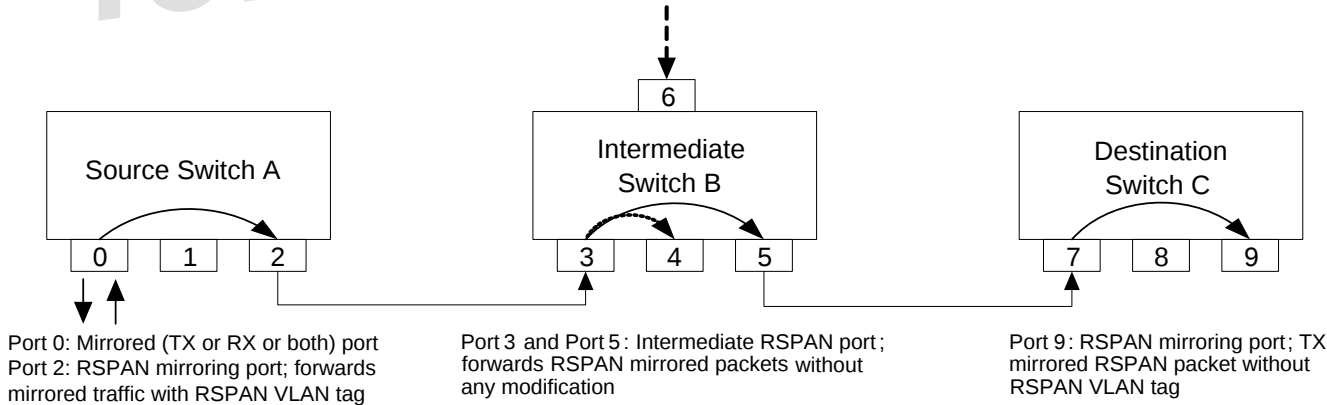
Figure 19. RSPAN Illustration
