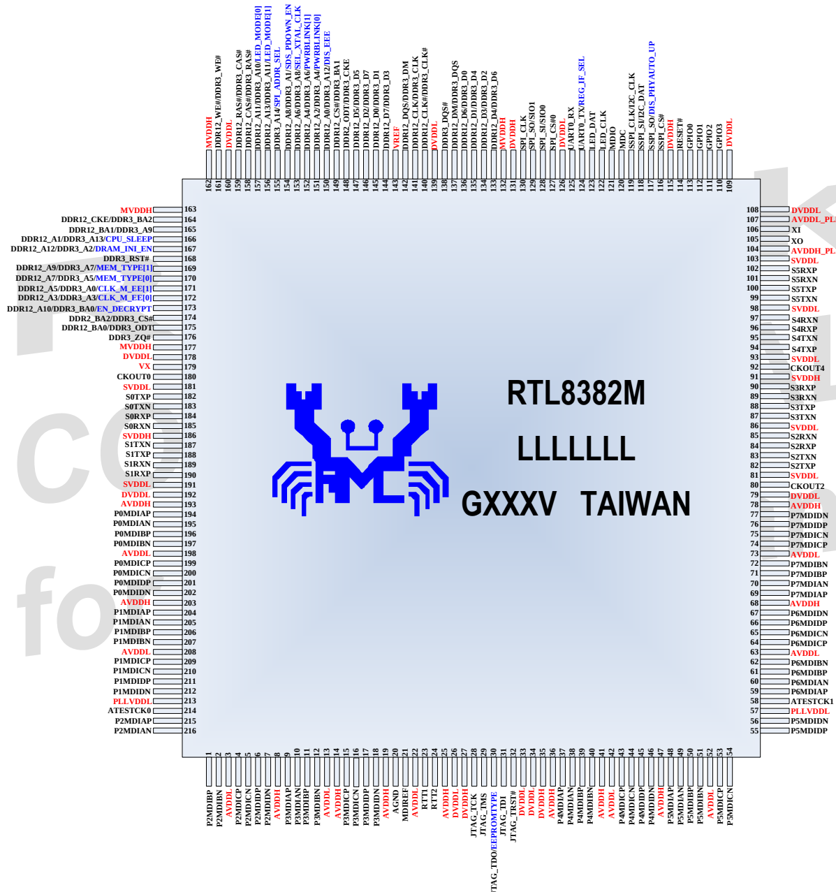
Figure 8. Pin Assignments (RTL8382M-VB)
