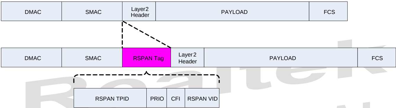
Figure 18. RSPAN Encapsulation
