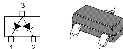
Marking Code: A1 SOT-23 Plastic Package
