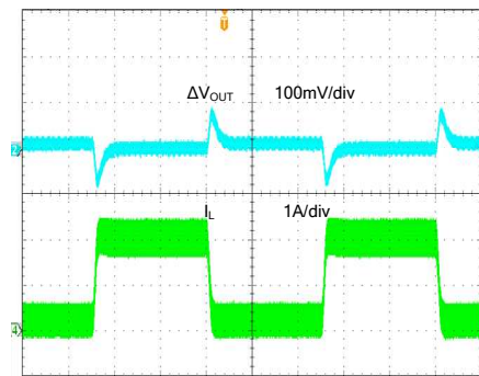
Load Transient ( V_{IN}=12V, V_{OUT}=3.3V, I_{LOAD}=0.2 \sim 2A )
