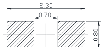
推荐焊盘尺寸 Recommended Soldering Pad
