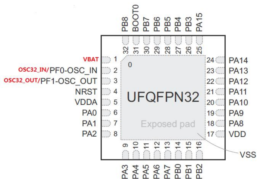
QFN28 封装 Pin-out
