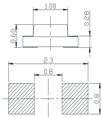
推荐焊盘尺寸 Recommended Soldering Pad
