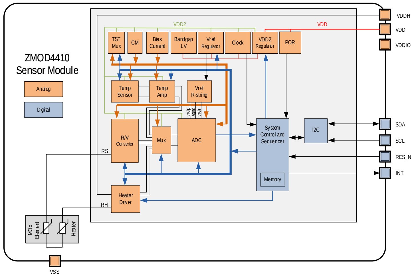
Figure 2. Block Diagram
