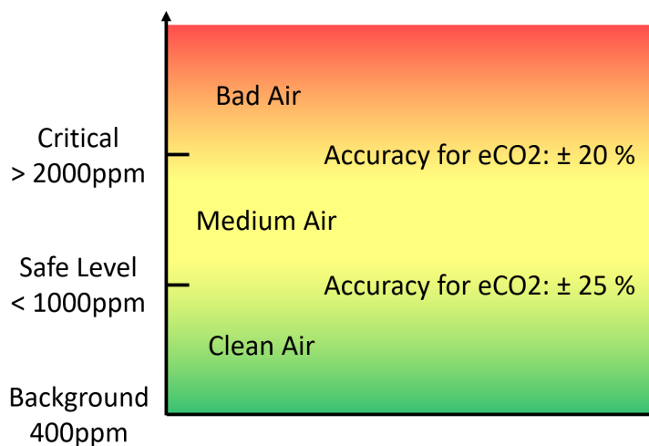
Figure 6. Concentration Dependent Accuracy for eCO 2
