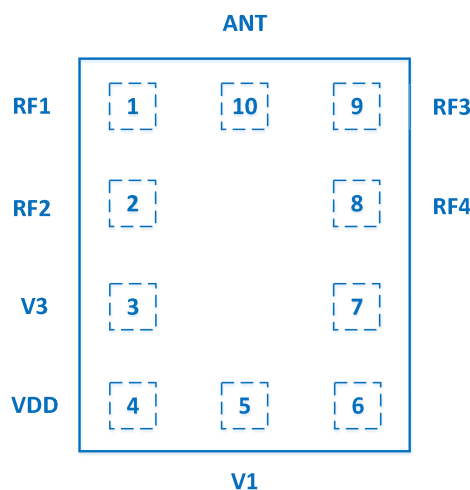
Figure 2 Pin-Out(Top View)
