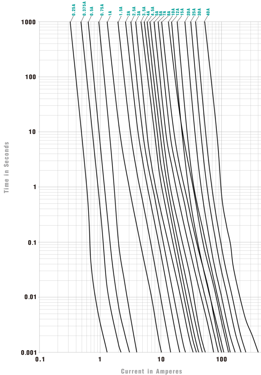
Average Time Current Curves
