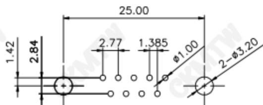
RECOMMENDED P.C.B LAYOUT (TOP VIEW)
