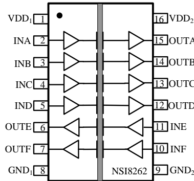
Figure 1.3 NSi8262 Package
