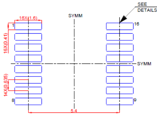
Figure 9.3 SSOP16 Package Shape and Dimension in millimeters
