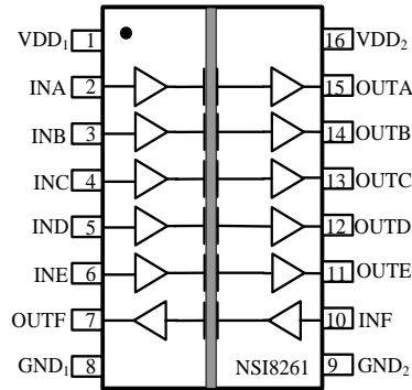
Figure 1.2 NSi8261 Package
