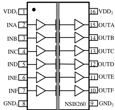
Figure 1.1 NSi8260 Package
