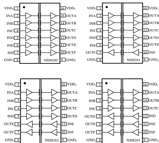
Figure 1. NSI826x Block Diagram
