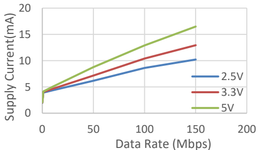
Figure 5.5 NSi8262 VDD1 Supply Current vs Data Rate
