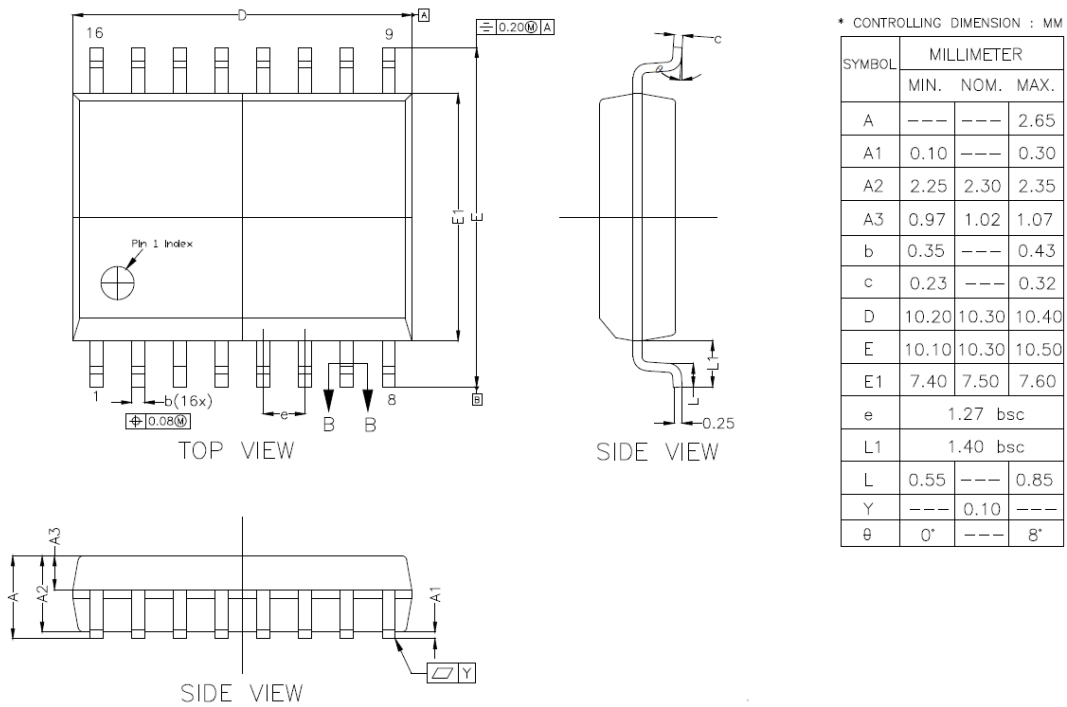
Figure 9.1 SOP16(300mil) Package Shape and Dimension in millimeters
