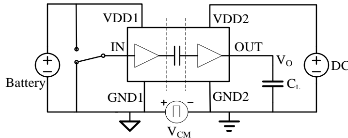
Figure 5.12 Common-Mode Transient Immunity Test Circuit
