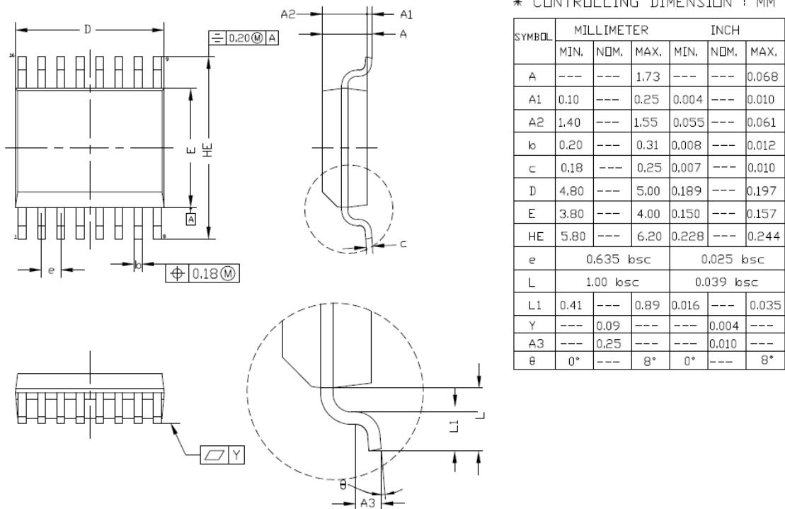
Figure 9.3 SSOP16 Package Shape and Dimension in millimeters
