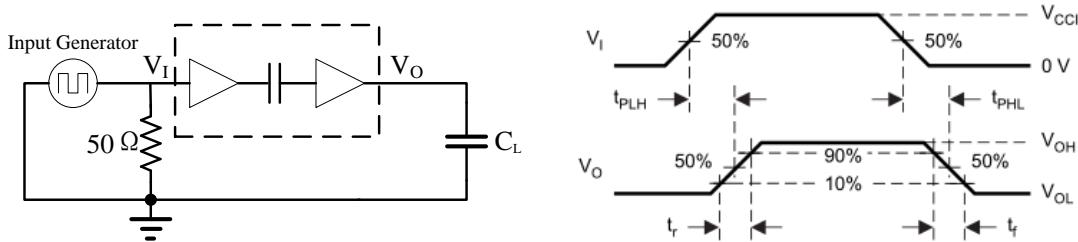
Figure 5.11 Switching Characteristics Test Circuit and Waveform
