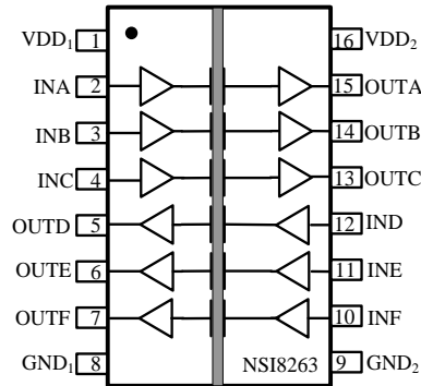
Figure 1.4 NSi8263 Package
